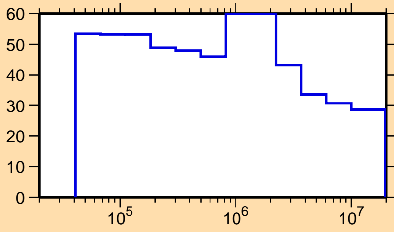
\Delta\sigma/\sigma vs. E for ^{163}\text{Yb}(n,n_1)
