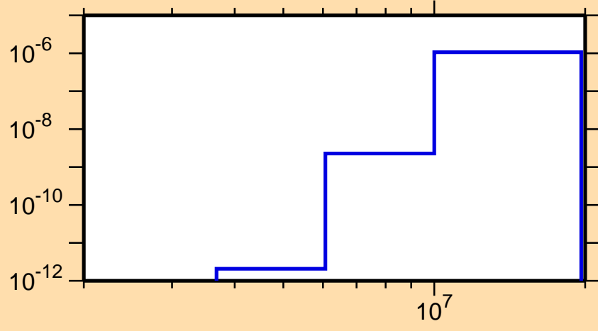
\sigma vs. E for ^{163}\text{Yb}(n,p\alpha)
