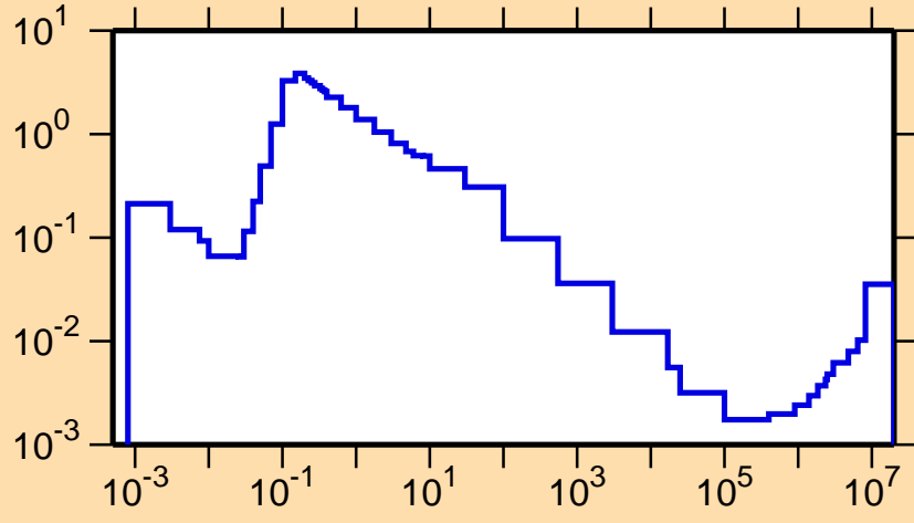
\sigma vs. E for ^{163}\text{Yb}(n,p)
