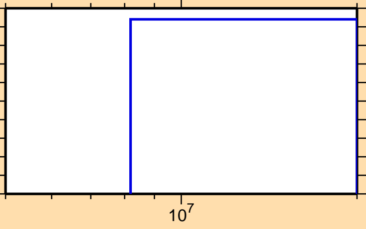
\sigma vs. E for ^{163}\text{Yb}(n,3n)
