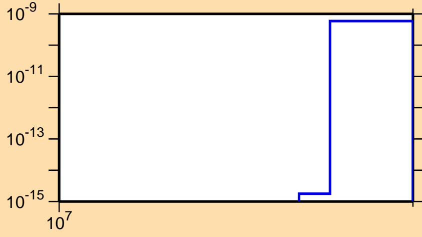
\sigma vs. E for ^{166}\text{Yb}(n,nt)
