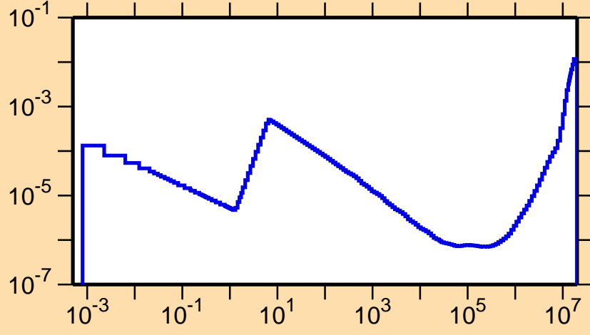
\sigma vs. E for ^{166}\text{Yb}(n,\alpha)
