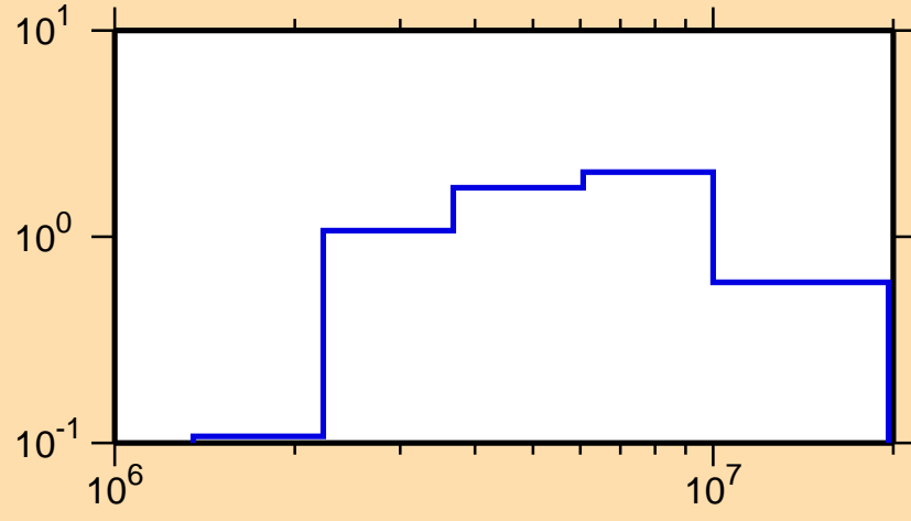
\sigma vs. E for ^{166}\text{Yb}(n,n\text{cont.})
