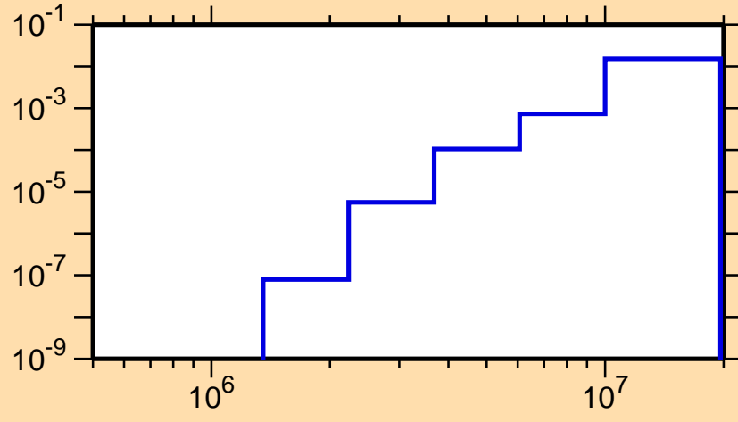
\sigma vs. E for ^{166}\text{Yb}(n,p)
