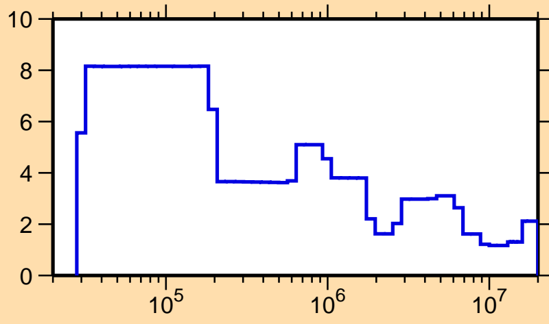
\Delta\sigma/\sigma vs. E for ^{167}\text{Yb}(n,\text{tot.})
