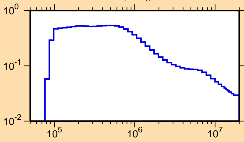
\sigma vs. E for ^{167}\text{Yb}(n,n_4)
