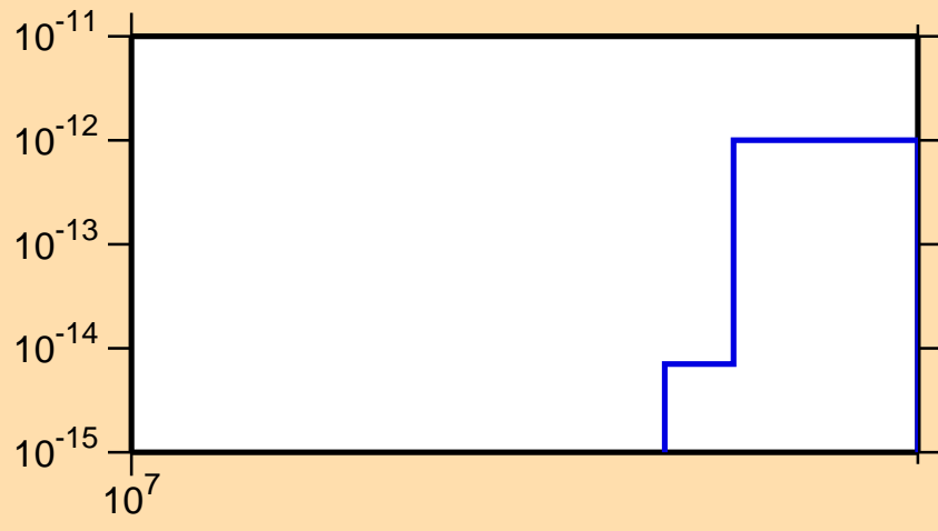
\sigma vs. E for ^{168}\text{Yb}(n,\text{pd})
