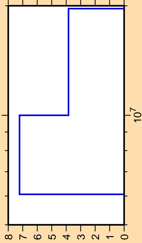
\Delta\sigma/\sigma vs. E for ^{168}\text{Yb}(n,2n)
