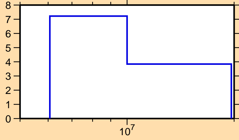
\Delta\sigma/\sigma vs. E for ^{168}\text{Yb}(n,2n)
