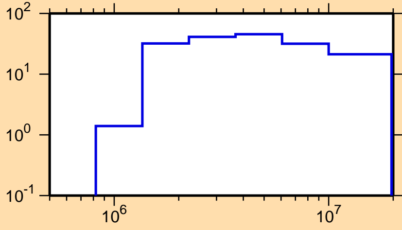
\Delta\sigma/\sigma vs. E for ^{168}\text{Yb}(n,p)
