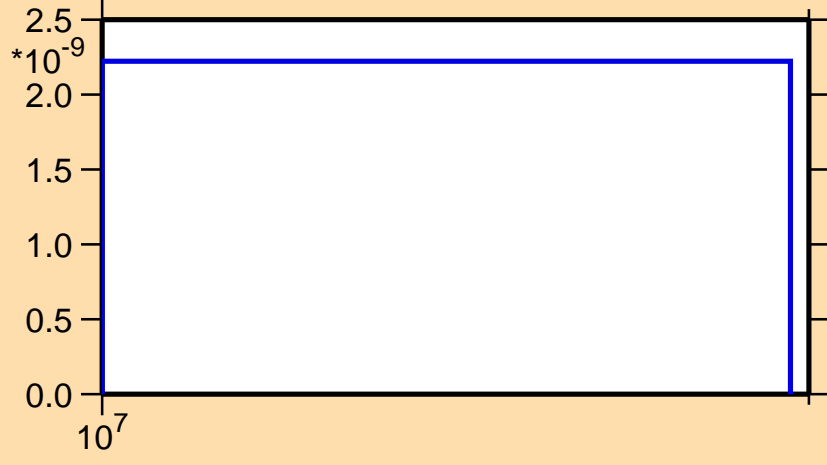
\sigma vs. E for ^{168}\text{Yb}(n,2n\alpha)
