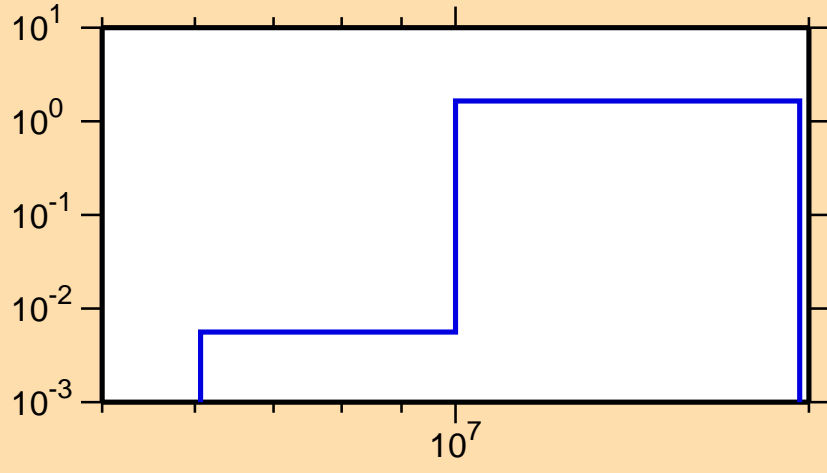
\sigma vs. E for ^{168}\text{Yb}(n,2n)
