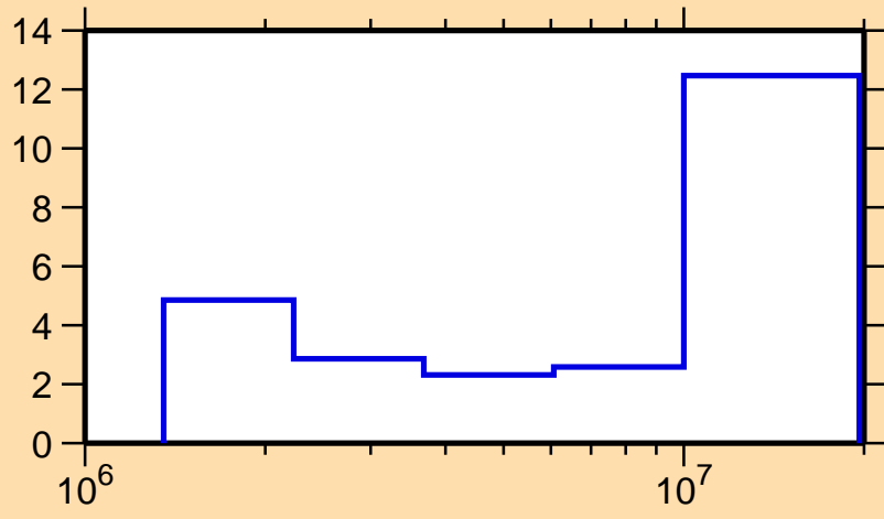
\Delta\sigma/\sigma vs. E for ^{168}\text{Yb}(n,n\text{cont.})
