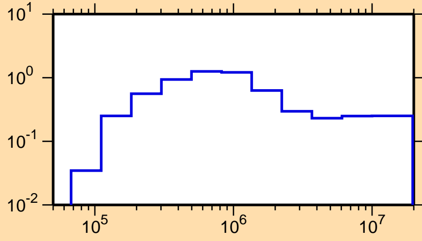
\sigma vs. E for ^{168}\text{Yb}(n,n_1)
