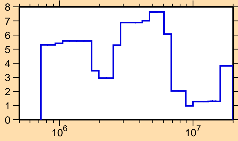
\Delta\sigma/\sigma vs. E for ^{169}\text{Yb}(n, el.)
