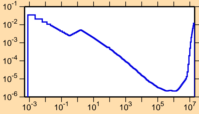
\sigma vs. E for ^{169}\text{Yb}(n,\alpha)
