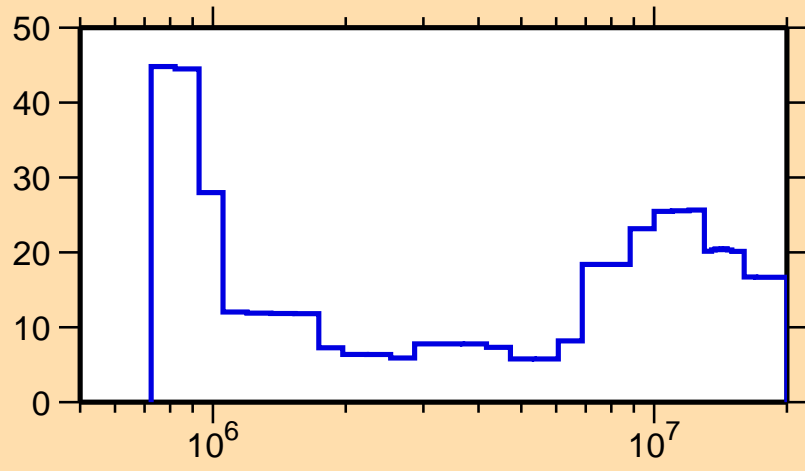
\Delta\sigma/\sigma vs. E for ^{169}\text{Yb}(n,n\text{cont.})
