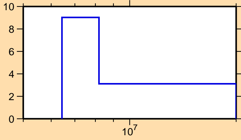
\Delta\sigma/\sigma vs. E for ^{171}\text{Yb}(n,2n)
