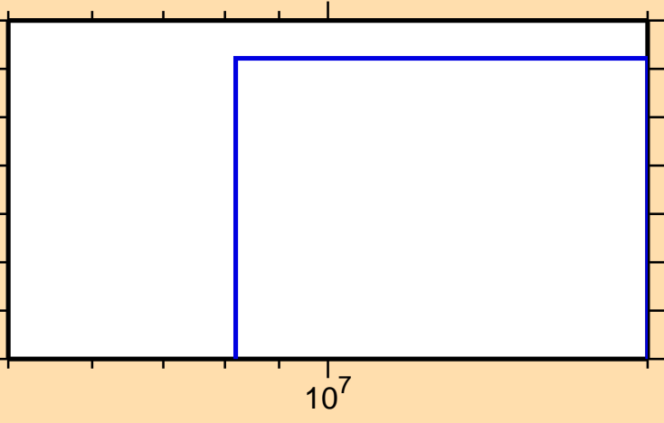
\sigma vs. E for ^{171}\text{Yb}(n,t)
