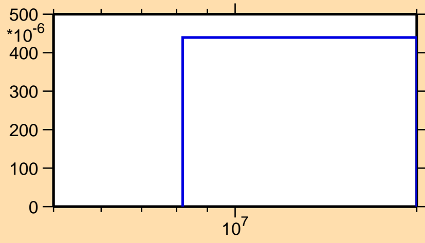
\sigma vs. E for ^{171}\text{Yb}(n,np)
