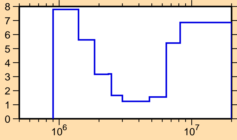
\Delta\sigma/\sigma vs. E for ^{171}\text{Yb}(n, \text{inel.})
