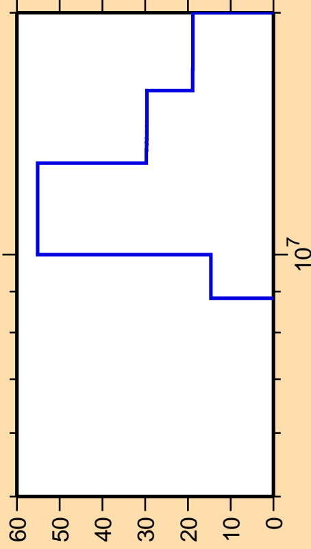
\Delta\sigma/\sigma vs. E for ^{172}\text{Yb}(n,np)
