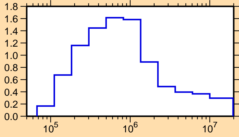
\sigma vs. E for ^{172}\text{Yb}(n,n_1)
