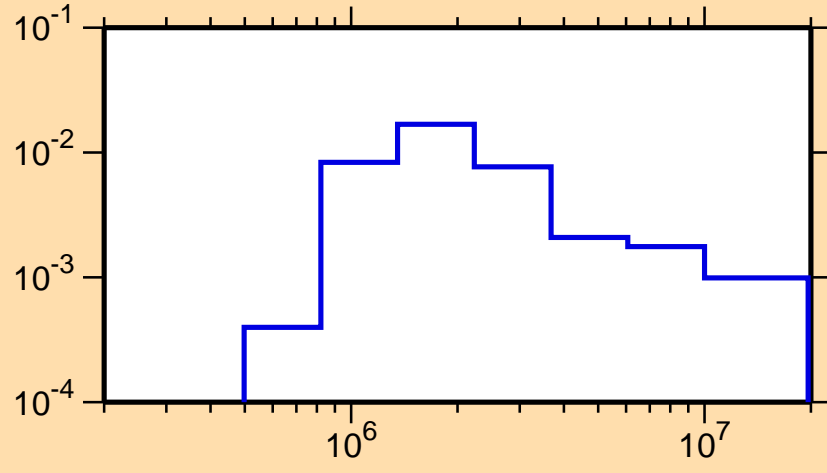
\sigma vs. E for ^{172}\text{Yb}(n,n_3)
