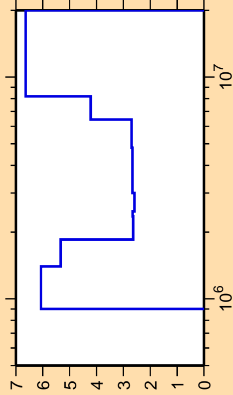
\Delta\sigma/\sigma vs. E for ^{173}\text{Yb}(n, ncont.)
