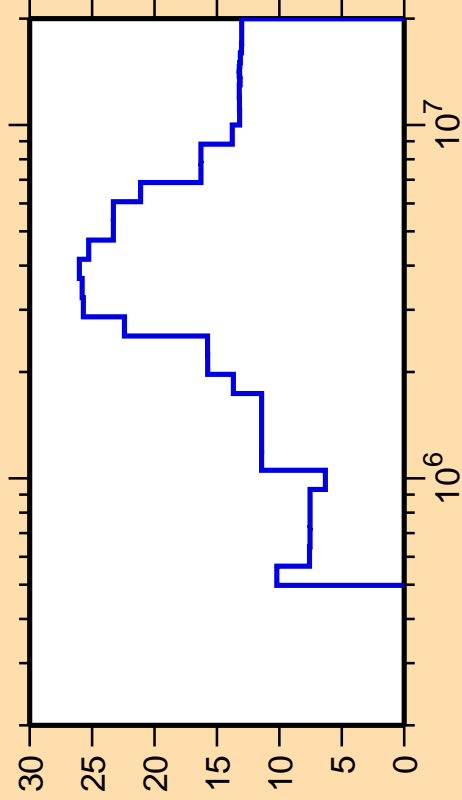
\Delta\sigma/\sigma vs. E for ^{174}\text{Yb}(n,n_3)
