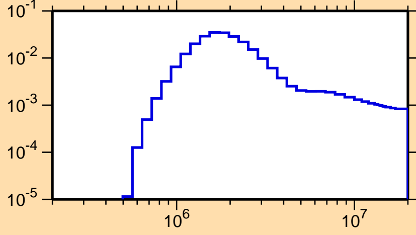
\sigma vs. E for ^{174}\text{Yb}(n,n_3)
