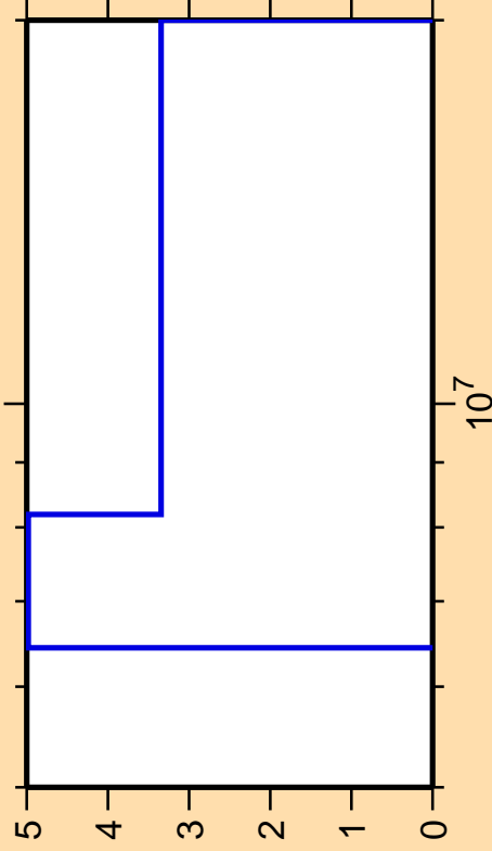
\Delta\sigma/\sigma vs. E for ^{174}\text{Yb}(n,2n)
