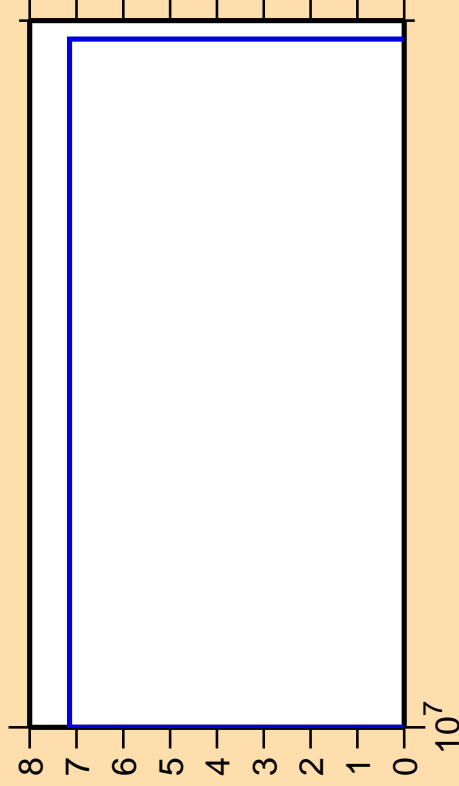
\Delta\sigma/\sigma vs. E for ^{175}\text{Yb}(n,3n)
