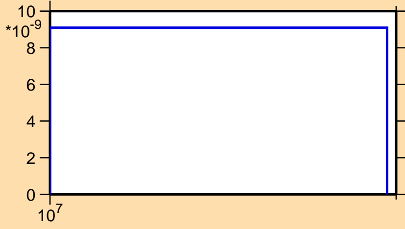
\sigma vs. E for ^{175}\text{Yb}(n,\text{nd})
