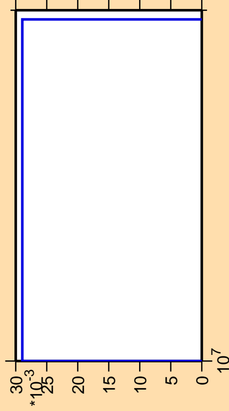
\Delta\sigma/\sigma vs. E for ^{175}\text{Yb}(n,\text{He}3)
