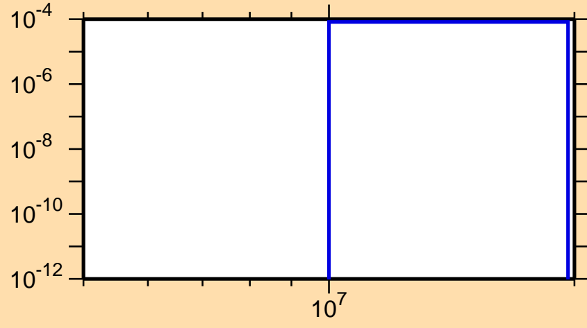
\sigma vs. E for ^{175}\text{Yb}(n,np)
