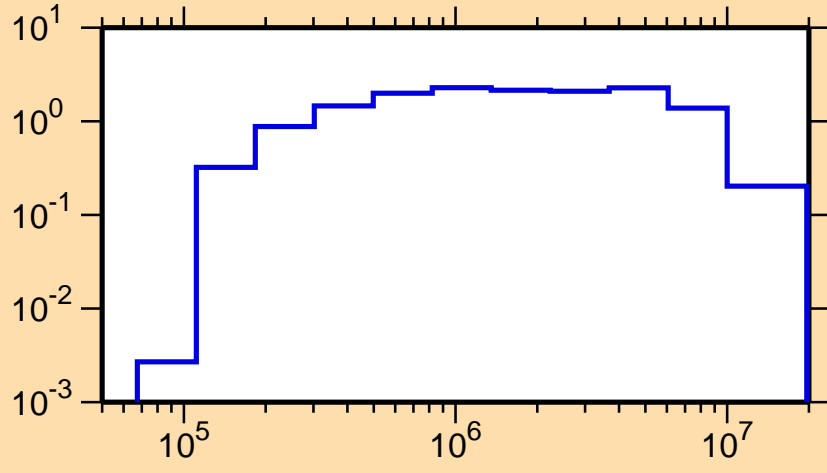
\sigma vs. E for ^{175}\text{Yb}(n,\text{inel.})
