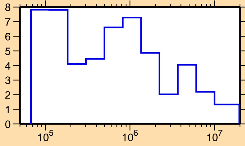
\Delta\sigma/\sigma vs. E for ^{175}\text{Yb}(n,\text{tot.})
