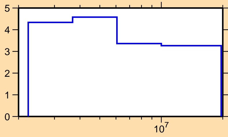
\Delta\sigma/\sigma vs. E for ^{175}\text{Yb}(n,\text{nonel.})
