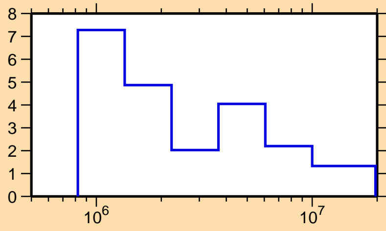
\Delta\sigma/\sigma vs. E for ^{175}\text{Yb}(n, tot.)
