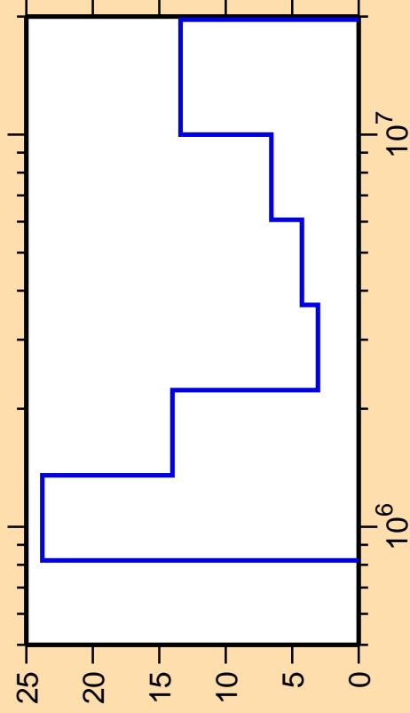
\Delta\sigma/\sigma vs. E for ^{175}\text{Yb}(n, ncont.)
