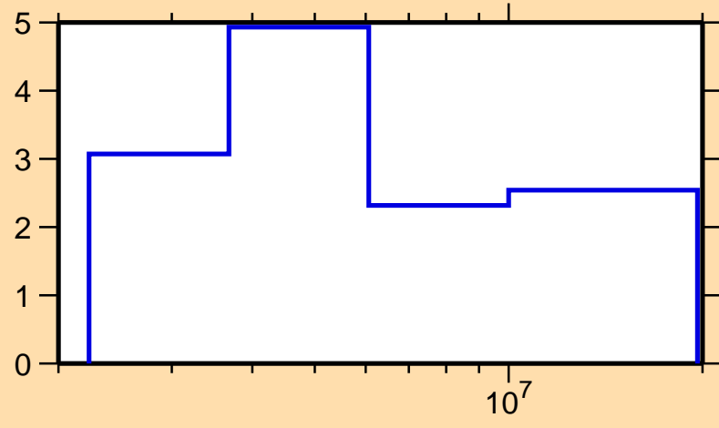
\Delta\sigma/\sigma vs. E for ^{175}\text{Yb}(n,\text{el.})
