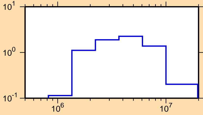
\sigma vs. E for ^{175}\text{Yb}(n,n\text{cont.})
