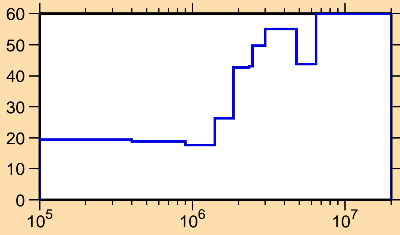
\Delta\sigma/\sigma vs. E for ^{175}\text{Yb}(n,n_1)
