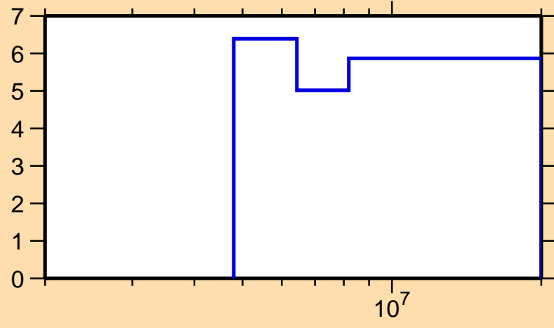
\Delta\sigma/\sigma vs. E for ^{175}\text{Yb}(n,2n)
