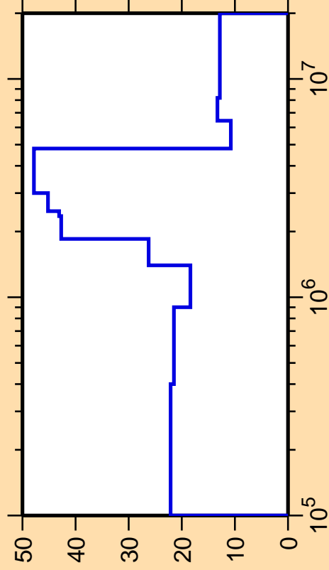
\Delta\sigma/\sigma vs. E for ^{175}\text{Yb}(n,n_2)
