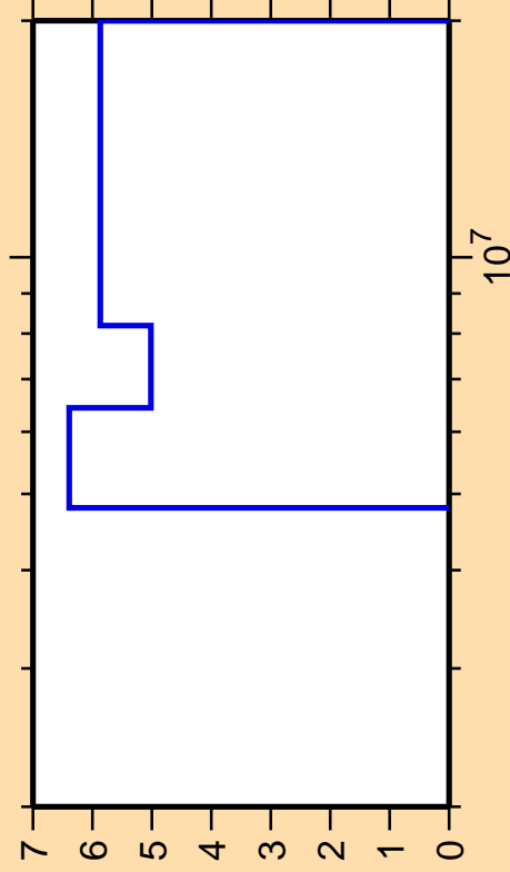
\Delta\sigma/\sigma vs. E for ^{175}\text{Yb}(n,2n)
