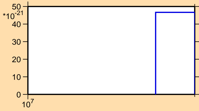
\sigma vs. E for ^{178}\text{Yb} (mt 11)
