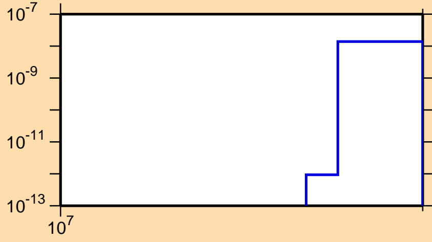
\sigma vs. E for ^{178}\text{Yb}(n,\text{nd})
