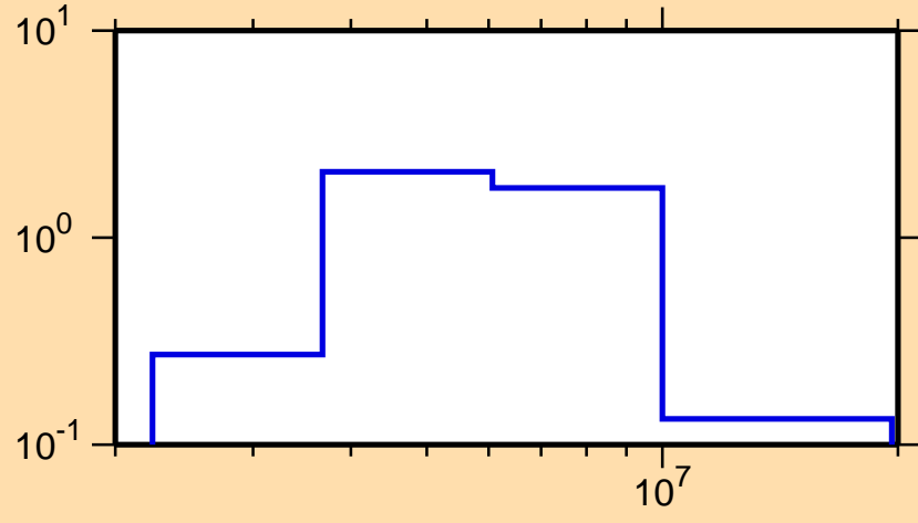
\sigma vs. E for ^{178}\text{Yb}(n,n\text{cont.})
