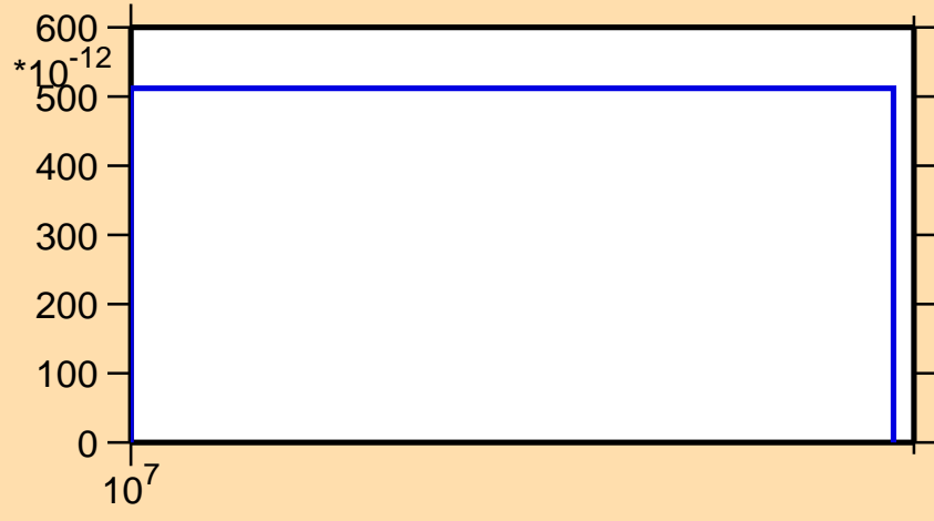
\sigma vs. E for ^{178}\text{Yb}(n,nt)
