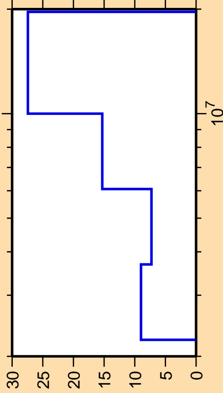
\Delta\sigma/\sigma vs. E for ^{178}\text{Yb}(n,n\text{cont.})
