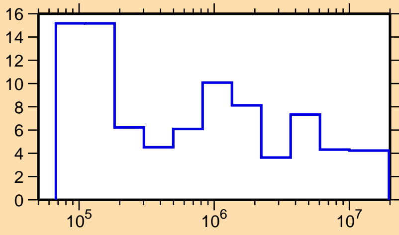
\Delta\sigma/\sigma vs. E for ^{178}\text{Yb}(n,\text{el.})
