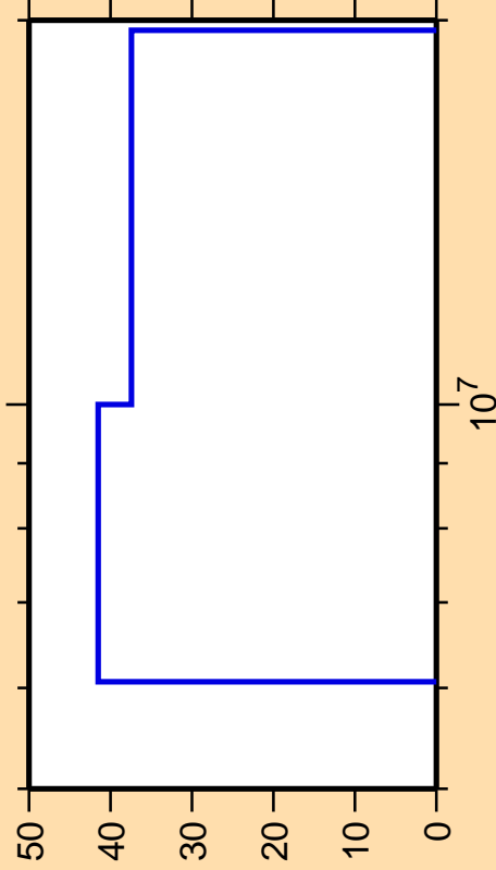
\Delta\sigma/\sigma vs. E for ^{178}\text{Yb}(n,p)
