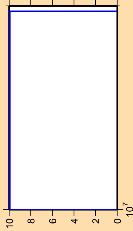
\Delta\sigma/\sigma vs. E for ^{178}\text{Yb}(n,3n)
