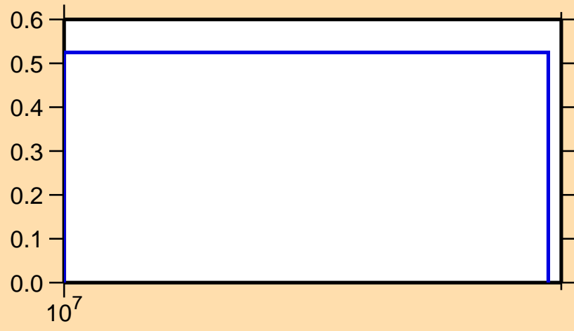
\sigma vs. E for ^{178}\text{Yb}(n,3n)
