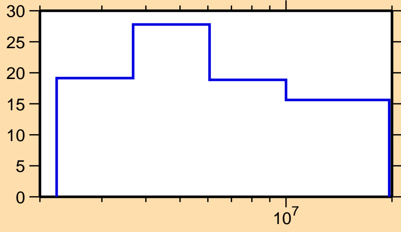
\Delta\sigma/\sigma vs. E for ^{178}\text{Yb}(n,n_1)
