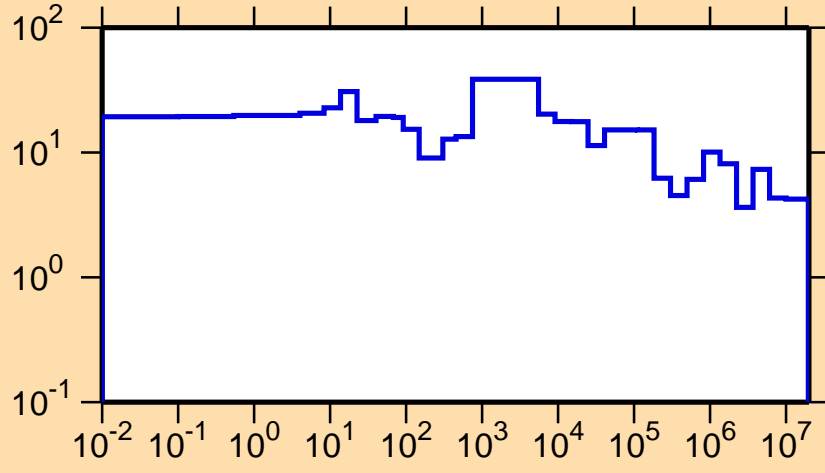
\Delta\sigma/\sigma vs. E for ^{178}\text{Yb}(n,\text{el.})
