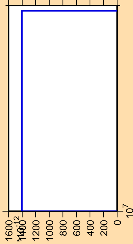
\Delta\sigma/\sigma vs. E for ^{178}\text{Yb} (mt 11)
