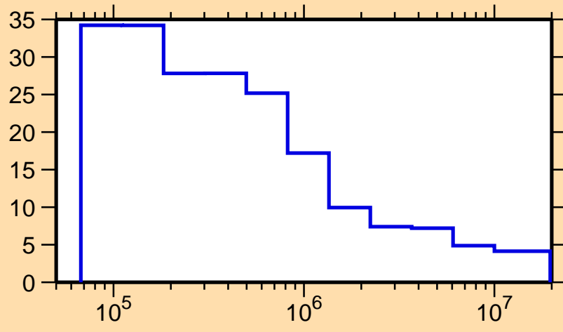
\Delta\sigma/\sigma vs. E for ^{178}\text{Yb}(n,\text{nonel.})
