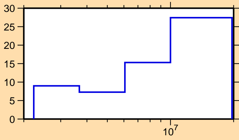
\Delta\sigma/\sigma vs. E for ^{178}\text{Yb}(n,n\text{cont.})
