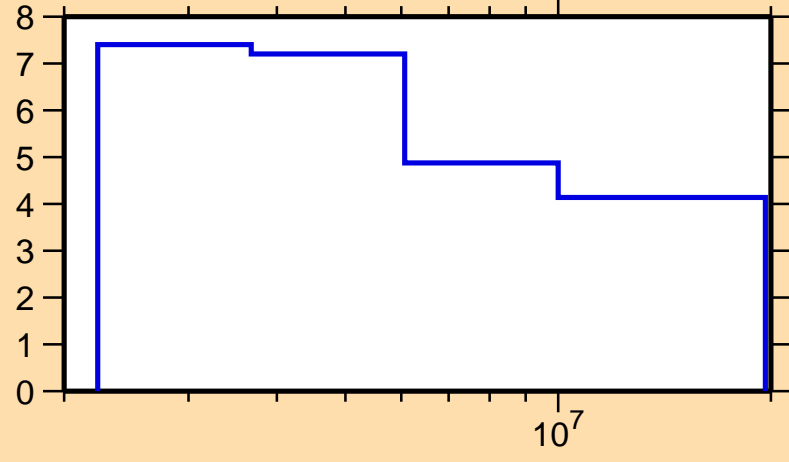
\Delta\sigma/\sigma vs. E for ^{178}\text{Yb}(n,\text{nonel.})
