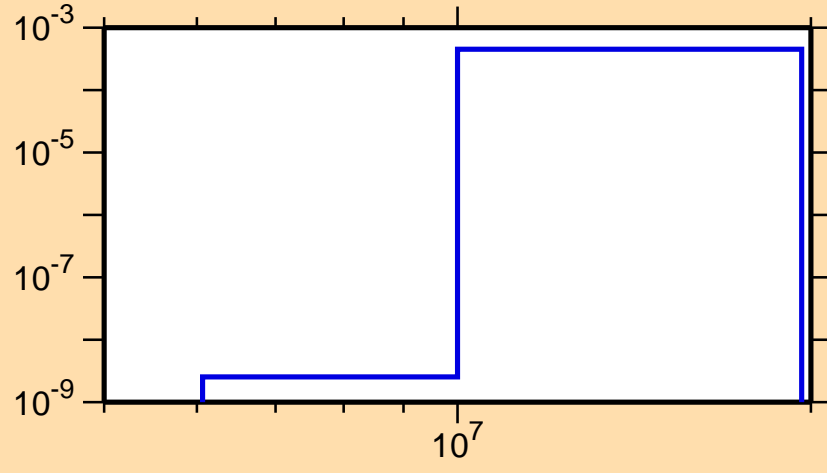
\sigma vs. E for ^{178}\text{Yb}(n,p)
