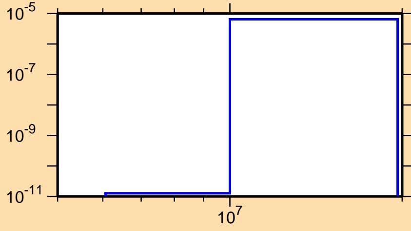
\sigma vs. E for ^{178}\text{Yb}(n,n\alpha)
