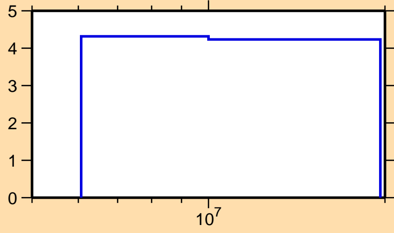
\Delta\sigma/\sigma vs. E for ^{178}\text{Yb}(n,\text{el.})
