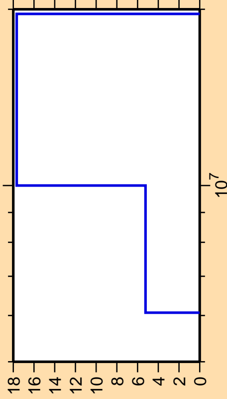
\Delta\sigma/\sigma vs. E for ^{178}\text{Yb}(n,2n)
