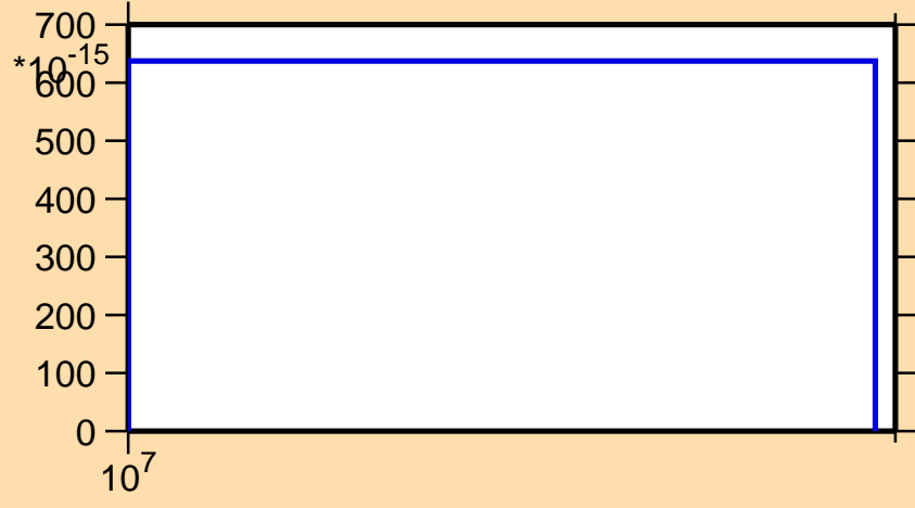
\sigma vs. E for ^{178}\text{Yb}(n,2np)
