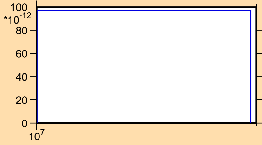
\sigma vs. E for ^{178}\text{Yb}(n,\text{nd})
