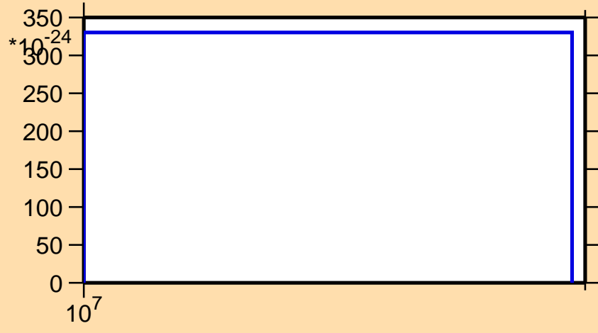
\sigma vs. E for ^{178}\text{Yb} (mt 11)
