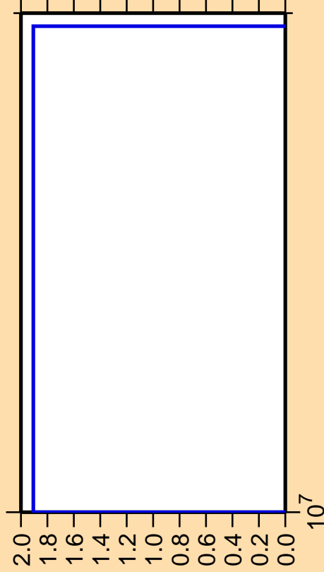
\Delta\sigma/\sigma vs. E for ^{178}\text{Yb}(n,2np)
