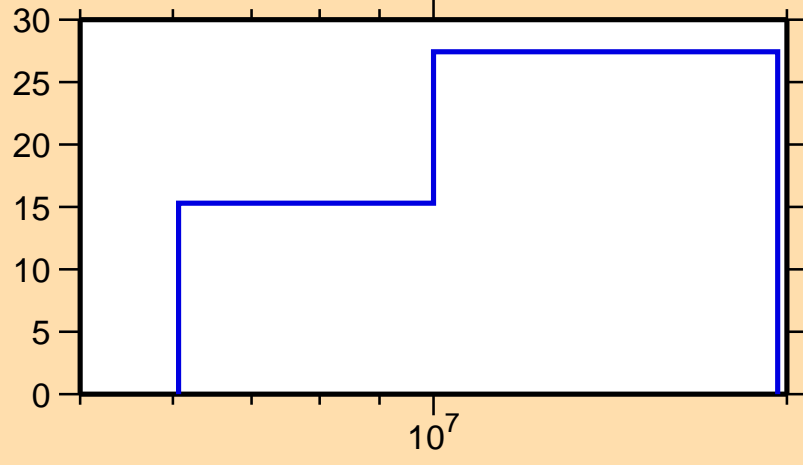
\Delta\sigma/\sigma vs. E for ^{178}\text{Yb}(n,n\text{cont.})
