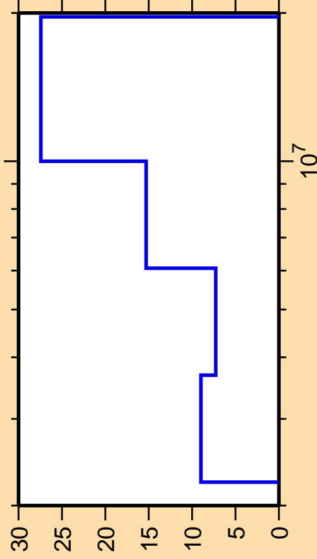
\Delta\sigma/\sigma vs. E for ^{178}\text{Yb}(n,n\text{cont.})
