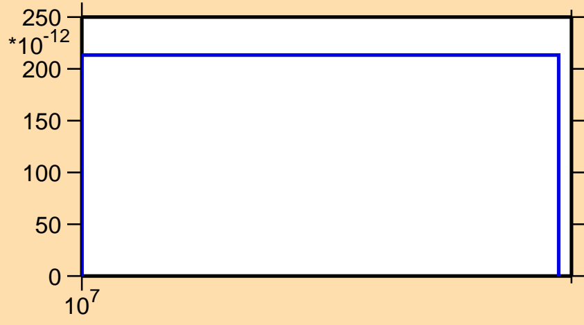
\sigma vs. E for ^{178}\text{Yb}(n,2n\alpha)
