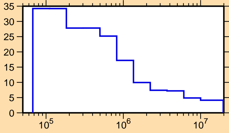
\Delta\sigma/\sigma vs. E for ^{178}\text{Yb}(n,\text{nonel.})
