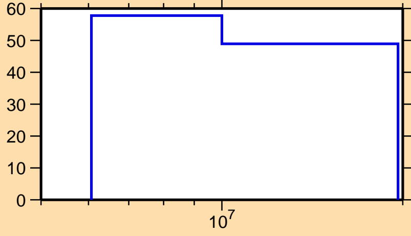
\Delta\sigma/\sigma vs. E for ^{178}\text{Yb}(n,\gamma)
