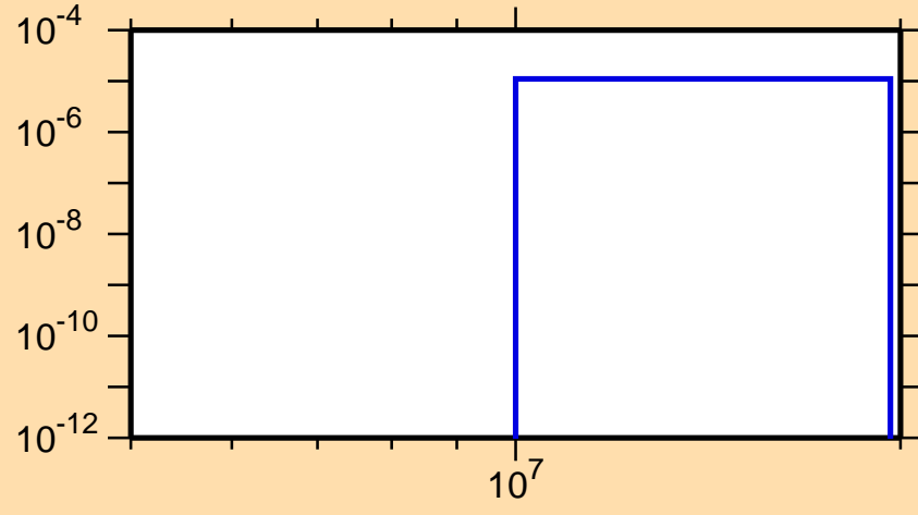
\sigma vs. E for ^{178}\text{Yb}(n,np)
