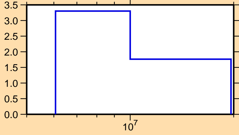
\Delta\sigma/\sigma vs. E for ^{178}\text{Yb}(n,\text{tot.})
