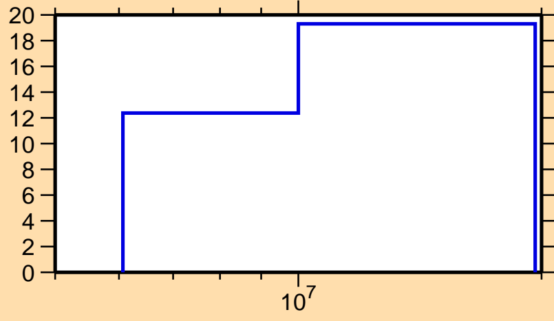
\Delta\sigma/\sigma vs. E for ^{178}\text{Yb}(n,\text{inel.})
