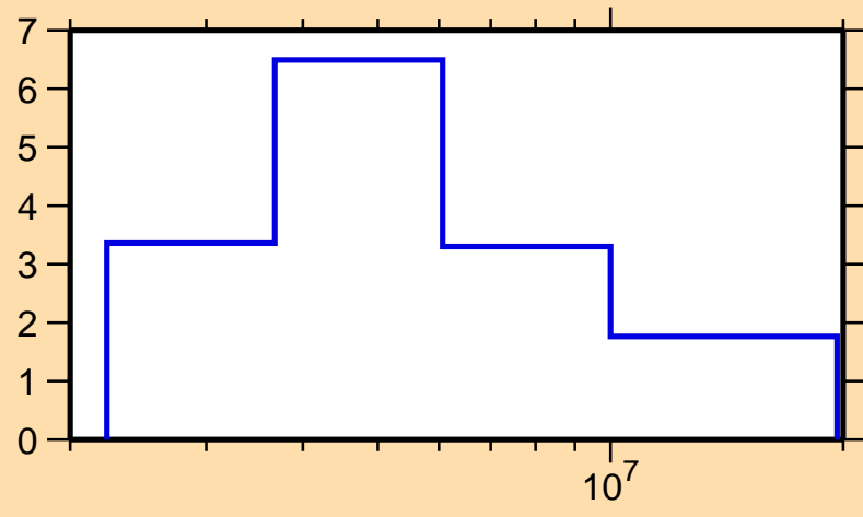
\Delta\sigma/\sigma vs. E for ^{178}\text{Yb}(n,\text{tot.})
