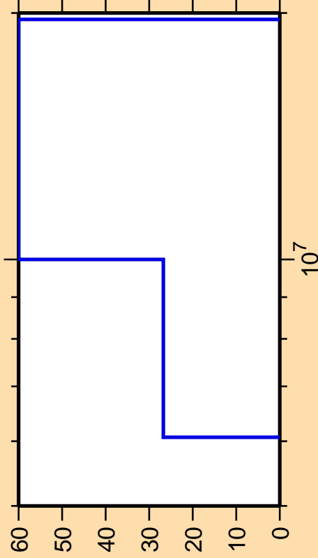
\Delta\sigma/\sigma vs. E for ^{178}\text{Yb}(n,n\alpha)
