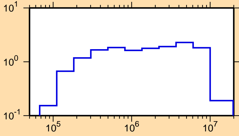
\sigma vs. E for ^{178}\text{Yb}(n,\text{inel.})
