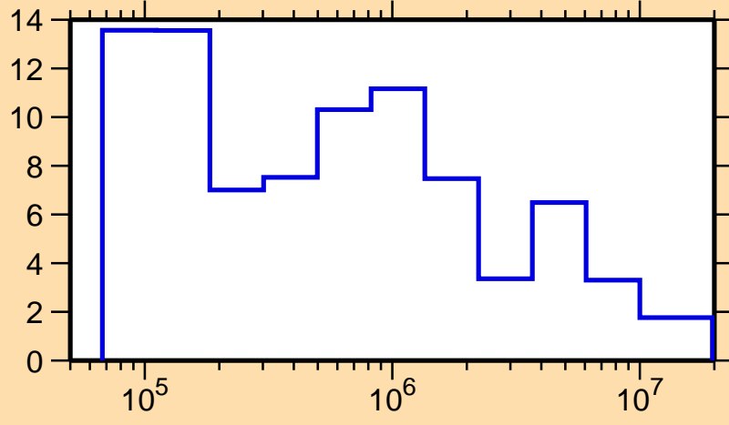
\Delta\sigma/\sigma vs. E for ^{178}\text{Yb}(n,\text{tot.})
