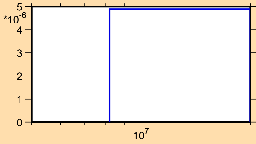
\sigma vs. E for ^{178}\text{Yb}(n,t)
