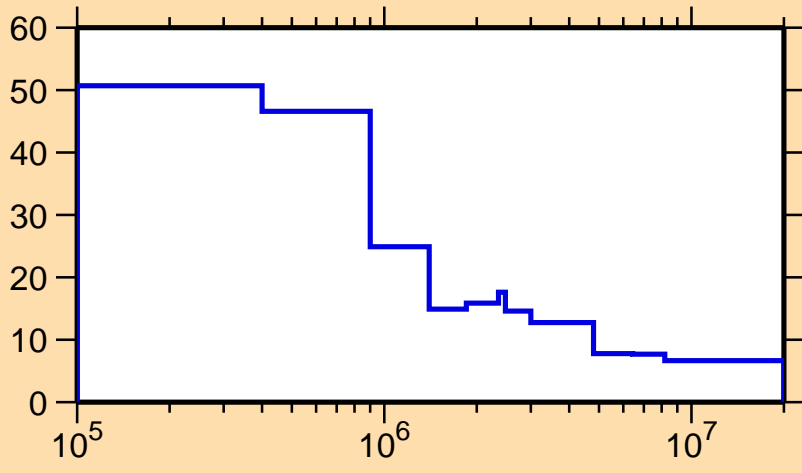
\Delta\sigma/\sigma vs. E for ^{180}\text{Yb}(n,\text{nonel.})
