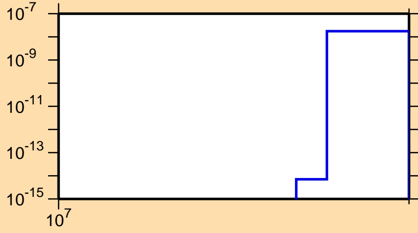
\sigma vs. E for ^{60}\text{Zn}(n,nd)
