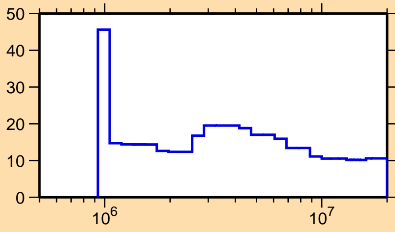
\Delta\sigma/\sigma vs. E for ^{60}\text{Zn}(n,n_1)
