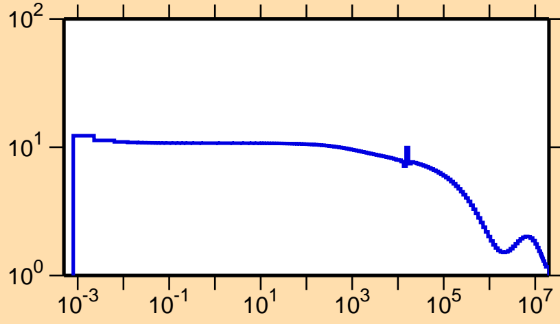
\sigma vs. E for ^{60}\text{Zn}(n,\text{el.})
