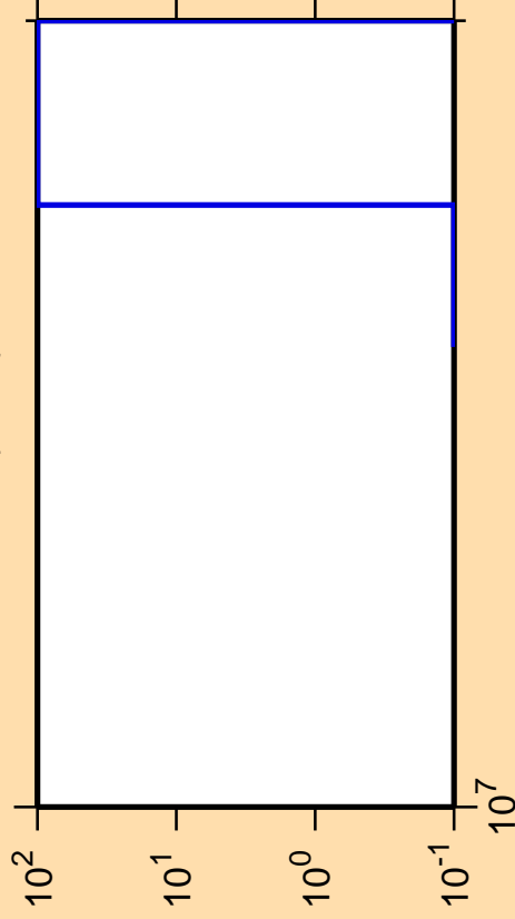
\Delta\sigma/\sigma vs. E for ^{60}\text{Zn}(n,nd)
