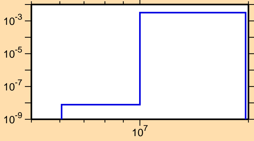
\sigma vs. E for ^{60}\text{Zn}(n,\text{pd})
