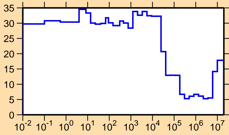
\Delta\sigma/\sigma vs. E for ^{60}\text{Zn}(n,p)
