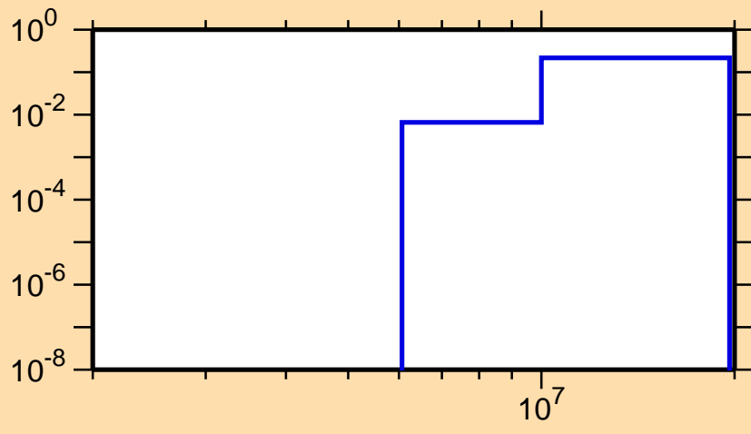
\sigma vs. E for ^{60}\text{Zn}(n,np)
