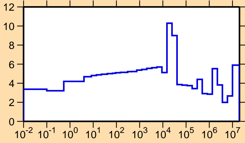
\Delta\sigma/\sigma vs. E for ^{60}\text{Zn}(n,\text{tot.})
