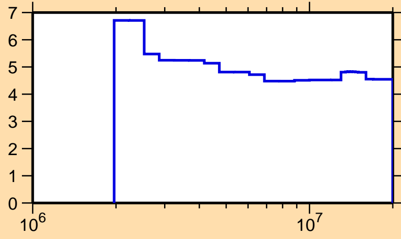
\Delta\sigma/\sigma vs. E for ^{61}\text{Zn}(n,n\text{onel.})
