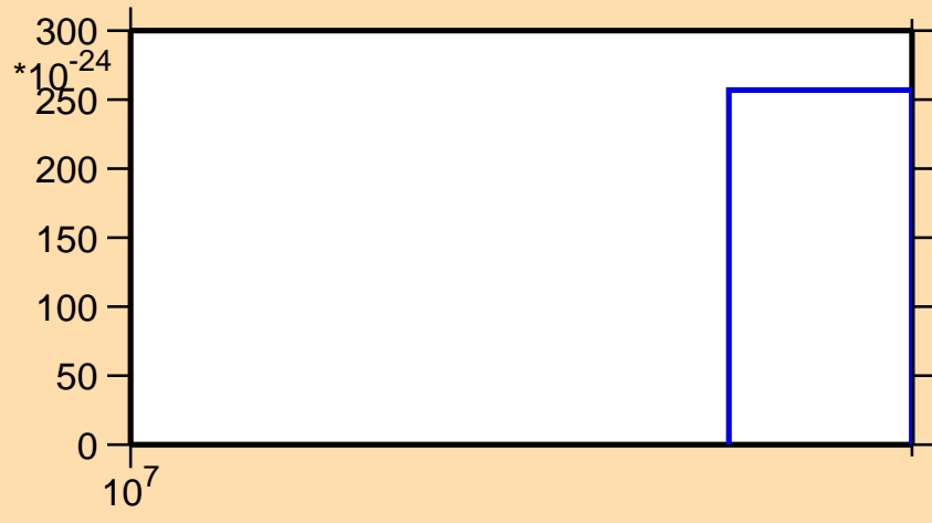
\sigma vs. E for ^{61}\text{Zn}(n,nt)
