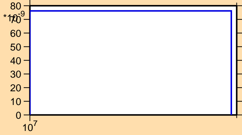
\sigma vs. E for ^{61}\text{Zn} (mt 34)
