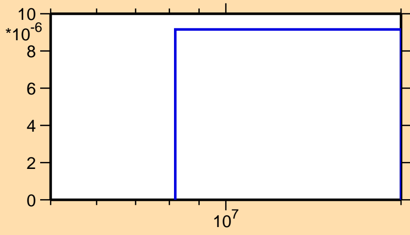
\sigma vs. E for ^{61}\text{Zn}(n,\text{pt})
