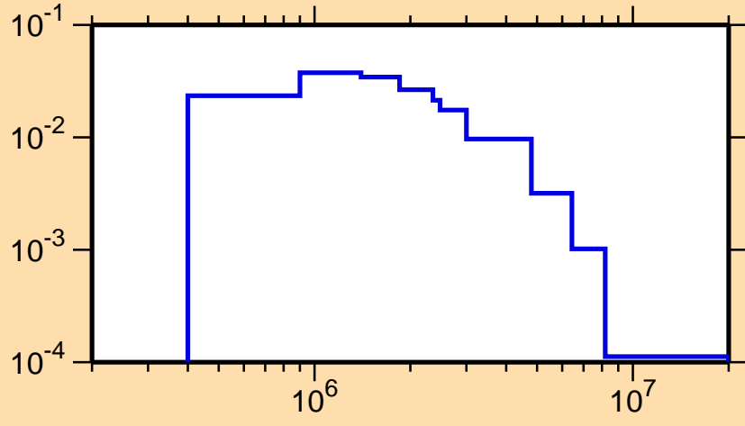
\sigma vs. E for ^{61}\text{Zn}(n,n_3)
