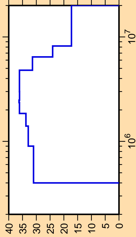
\Delta\sigma/\sigma vs. E for ^{61}\text{Zn}(n,n_3)
