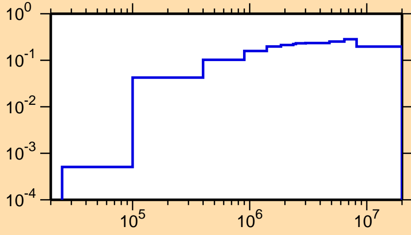
\sigma vs. E for ^{61}\text{Zn}(n,\text{inel.})
