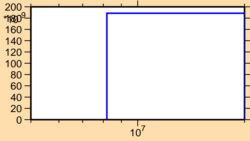
\sigma vs. E for ^{61}\text{Zn}(n,\text{nd})
