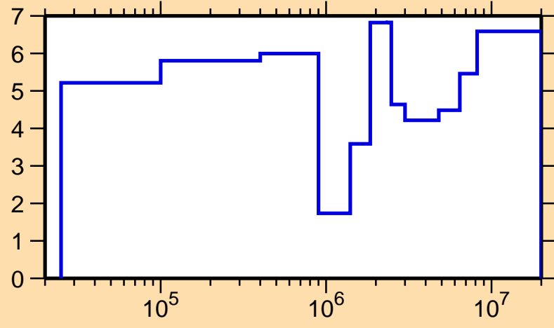
\Delta\sigma/\sigma vs. E for ^{61}\text{Zn}(n,\text{el.})
