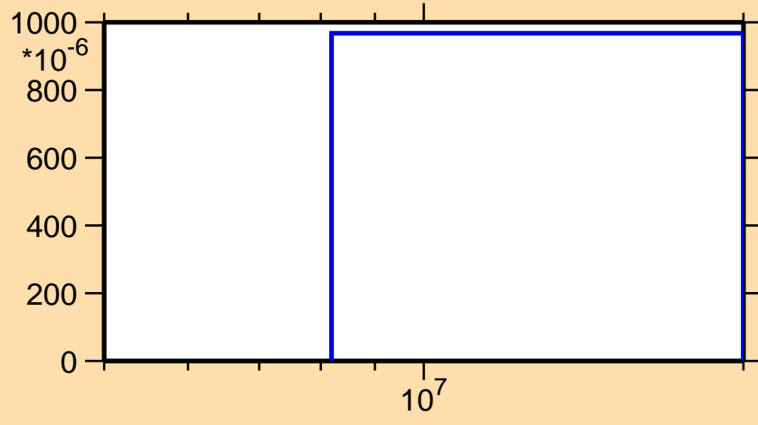
\sigma vs. E for ^{61}\text{Zn}(n,2n)
