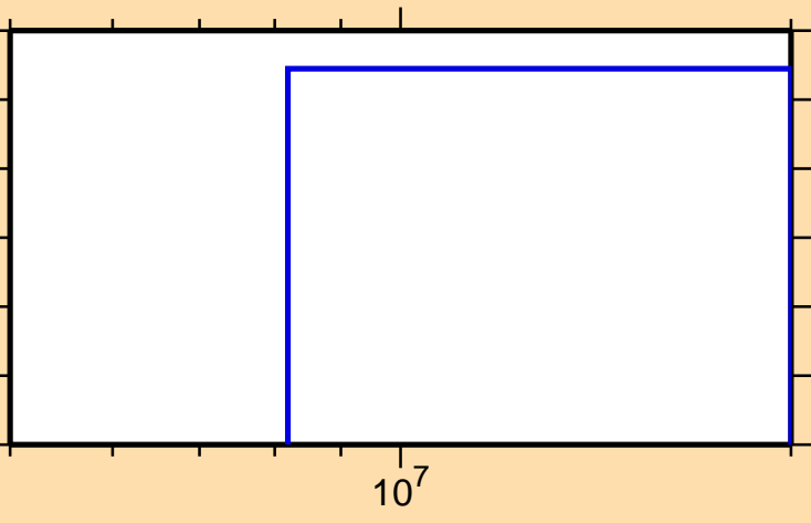
\sigma vs. E for ^{61}\text{Zn}(n,2n\alpha)
