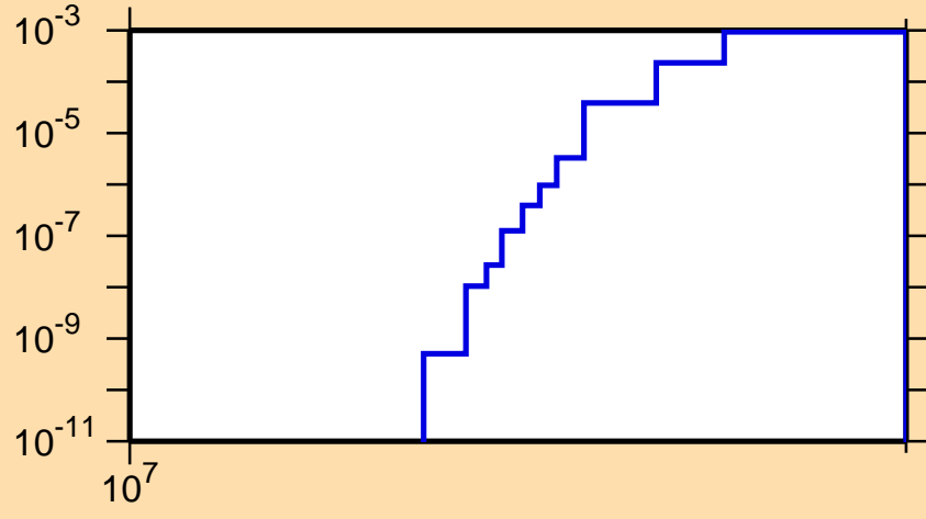
\sigma vs. E for ^{63}\text{Zn}(n,pd)
