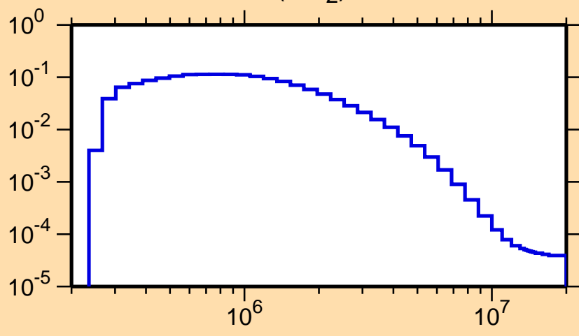
\sigma vs. E for ^{63}\text{Zn}(n,n_2)
