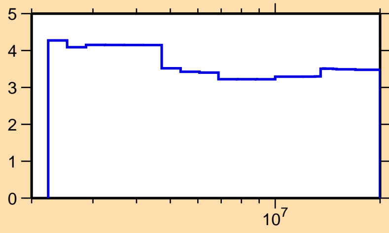
\Delta\sigma/\sigma vs. E for ^{63}\text{Zn}(n,n\text{onel.})
