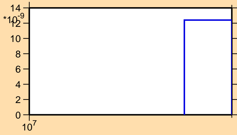
\sigma vs. E for ^{63}\text{Zn} (mt 45)
