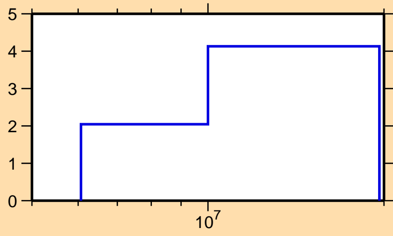
\Delta\sigma/\sigma vs. E for ^{63}\text{Zn}(n,\text{tot.})
