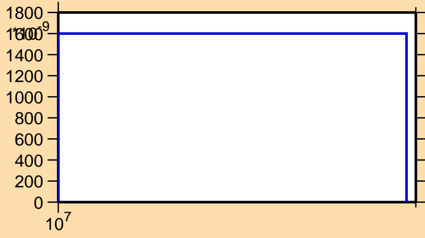
\sigma vs. E for ^{63}\text{Zn}(n,nd)
