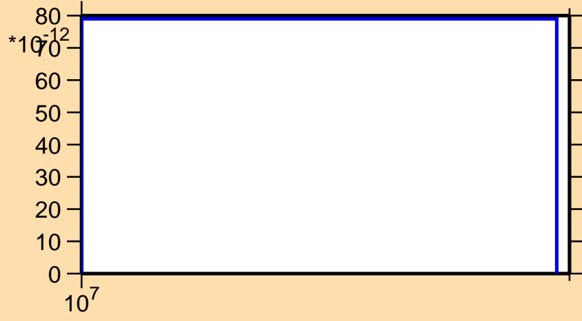
\sigma vs. E for ^{63}\text{Zn} (mt 45)
