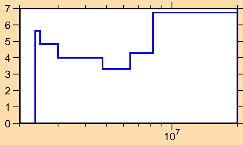
\Delta\sigma/\sigma vs. E for ^{63}\text{Zn}(n,\text{el.})
