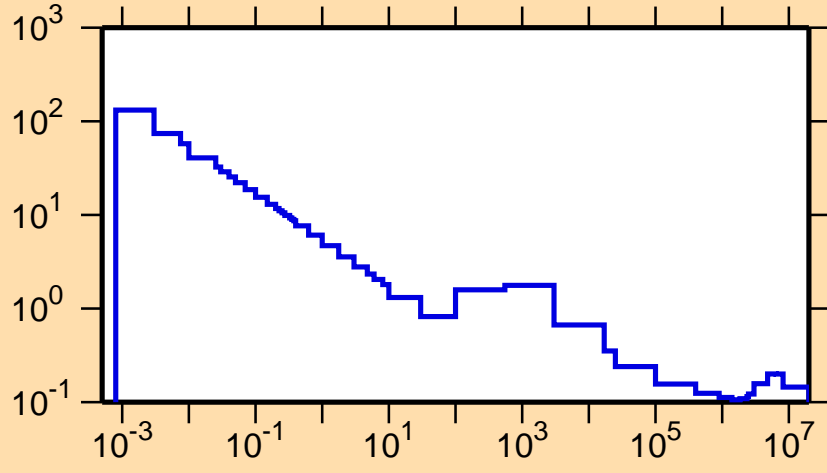
\sigma vs. E for ^{63}\text{Zn}(n,\alpha)
