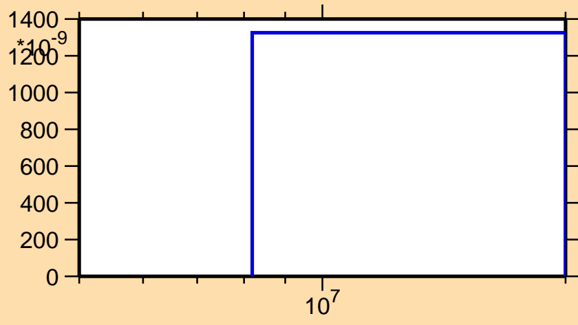
\sigma vs. E for ^{63}\text{Zn}(n,nd)
