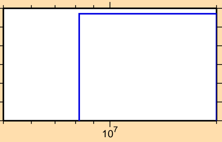
\sigma vs. E for ^{63}\text{Zn}(n,2n\alpha)
