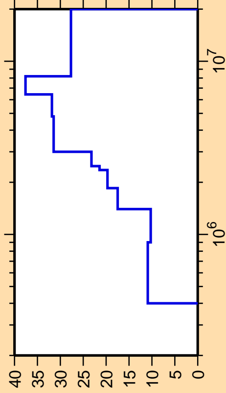
\Delta\sigma/\sigma vs. E for ^{63}\text{Zn}(n,n_4)
