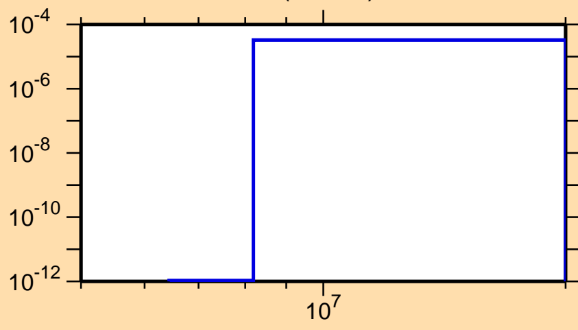
\sigma vs. E for ^{63}\text{Zn}(n,\text{He3})
