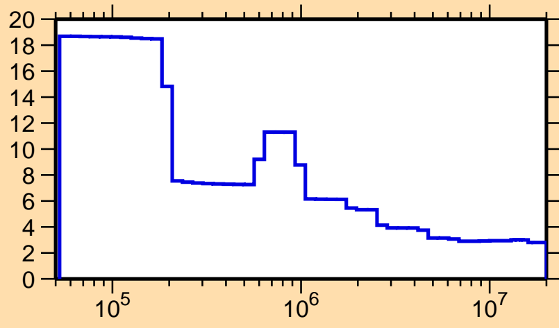
\Delta\sigma/\sigma vs. E for ^{65}\text{Zn}(n,\text{nonel.})
