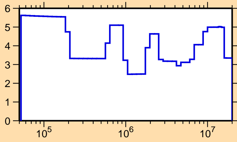
\Delta\sigma/\sigma vs. E for ^{65}\text{Zn}(n,\text{el.})
