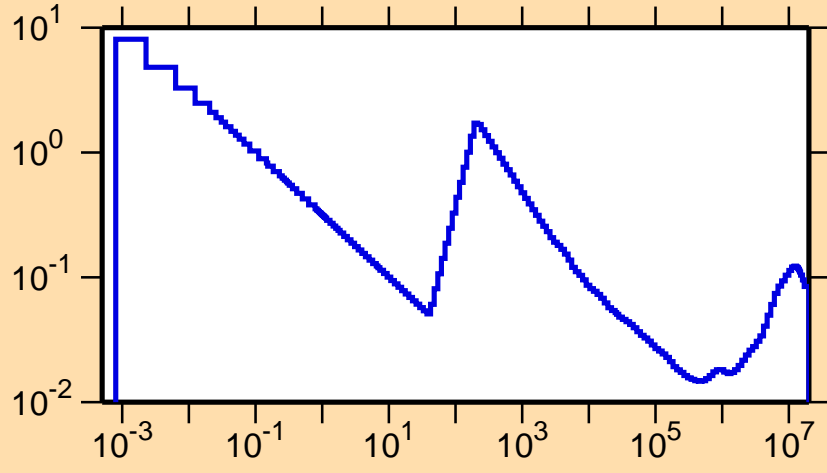
\sigma vs. E for ^{65}\text{Zn}(n,\alpha)
