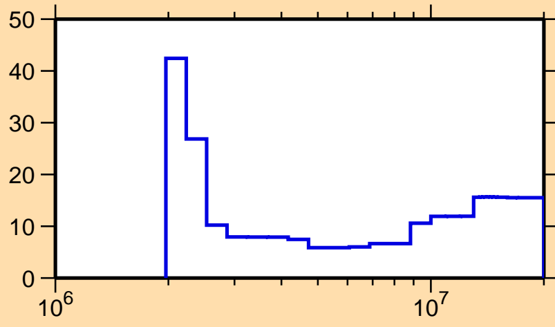
\Delta\sigma/\sigma vs. E for ^{65}\text{Zn}(n,n\text{cont.})
