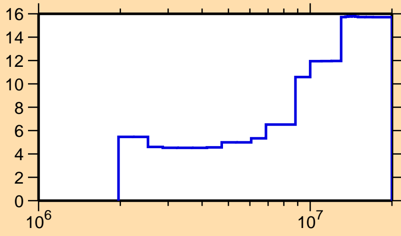
\Delta\sigma/\sigma vs. E for ^{65}\text{Zn}(n,\text{inel.})
