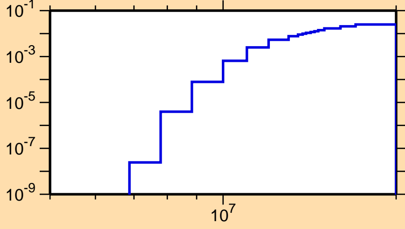
\sigma vs. E for ^{65}\text{Zn}(n,d)
