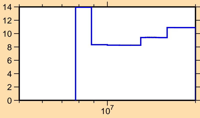
\Delta\sigma/\sigma vs. E for ^{65}\text{Zn}(n,2n)
