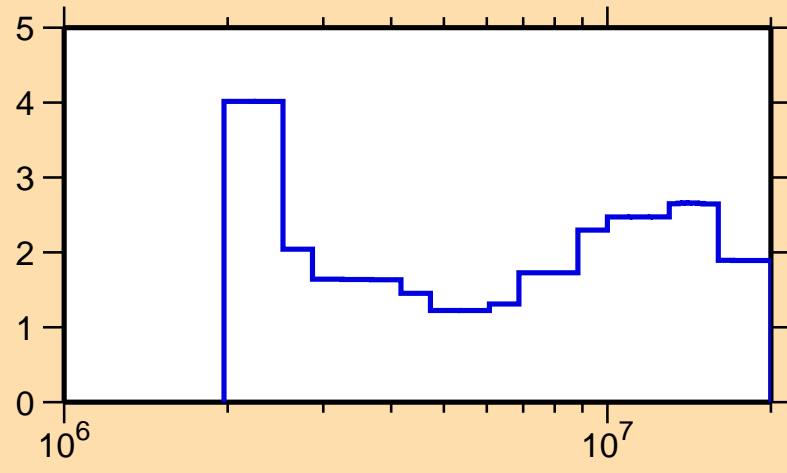
\Delta\sigma/\sigma vs. E for ^{65}\text{Zn}(n,\text{tot.})
