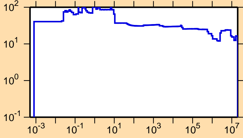
\Delta\sigma/\sigma vs. E for ^{65}\text{Zn}(n,p)
