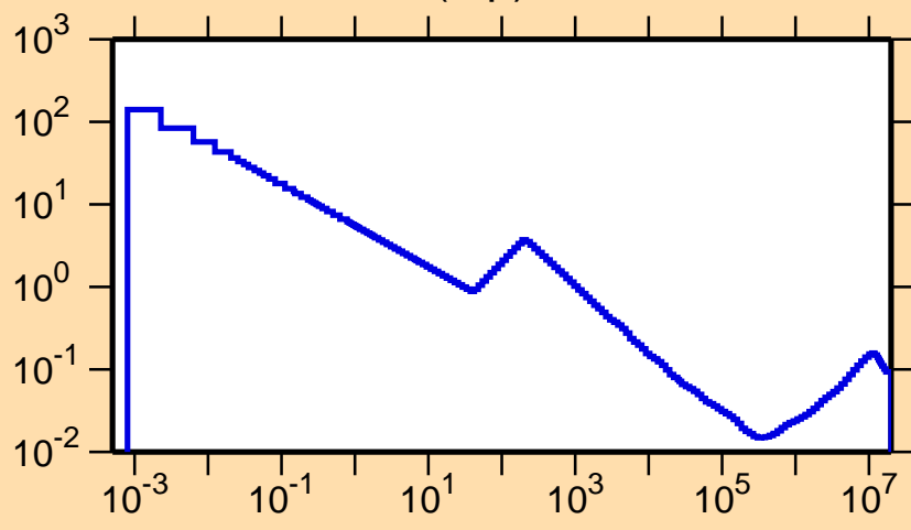
\sigma vs. E for ^{65}\text{Zn}(n,p)
