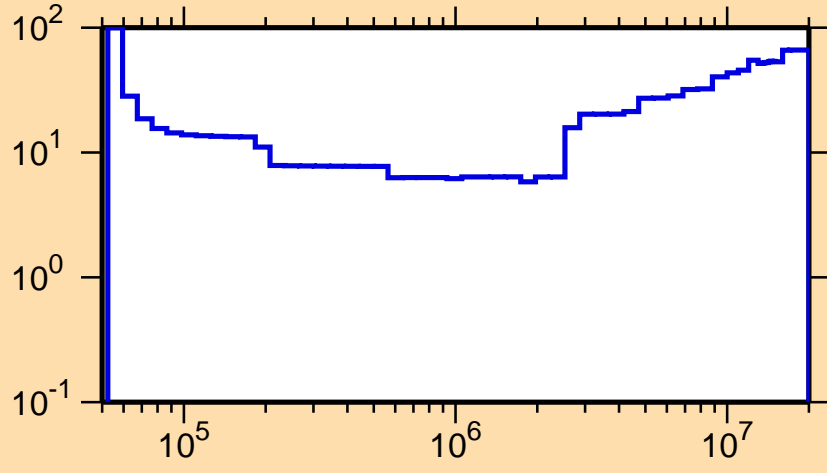
\Delta\sigma/\sigma vs. E for ^{65}\text{Zn}(n,n_1)
