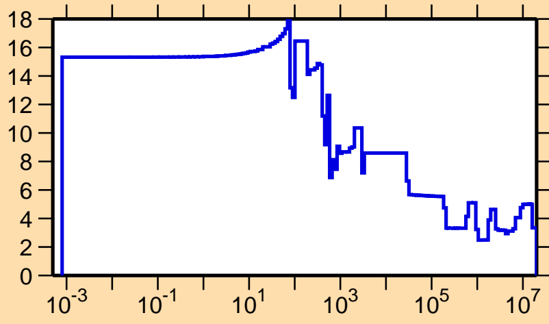
\Delta\sigma/\sigma vs. E for ^{65}\text{Zn}(n,\text{el.})
