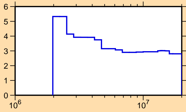
\Delta\sigma/\sigma vs. E for ^{65}\text{Zn}(n,n\text{onel.})
