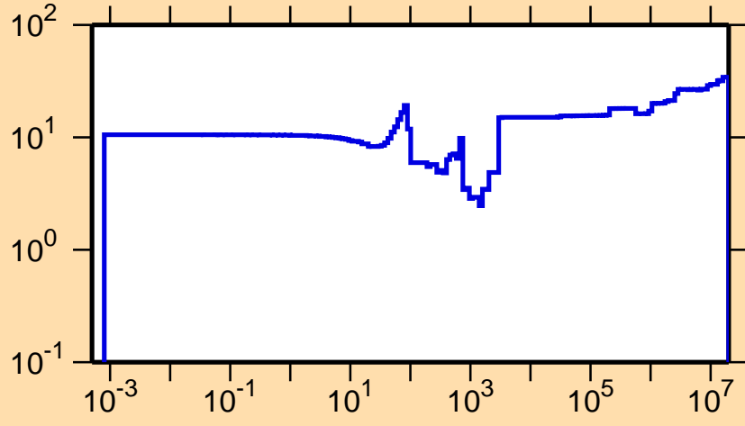
\Delta\sigma/\sigma vs. E for ^{65}\text{Zn}(n,\gamma)
