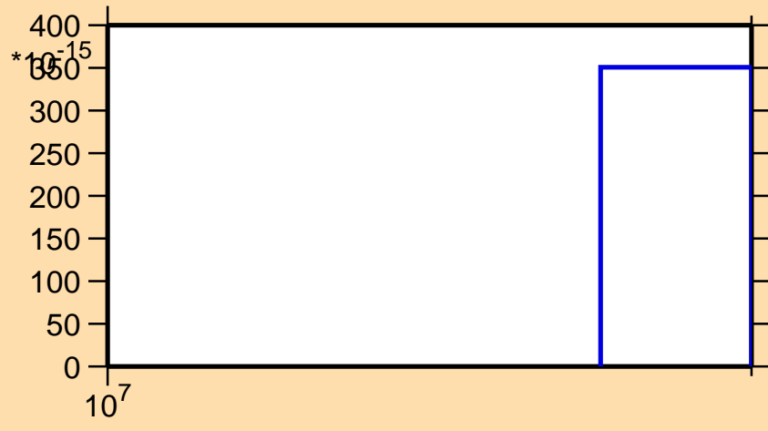
\sigma vs. E for ^{65}\text{Zn}(n,nt)
