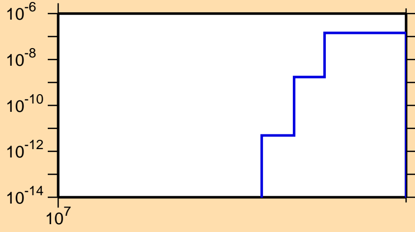
\sigma vs. E for ^{65}\text{Zn}(n,\text{pd})
