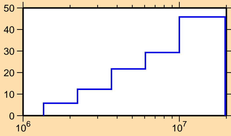
\Delta\sigma/\sigma vs. E for ^{65}\text{Zn}(n,n_1)
