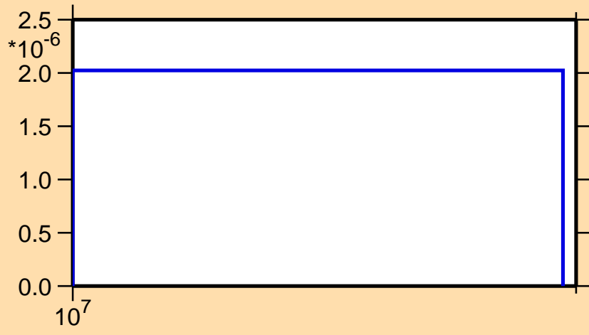
\sigma vs. E for ^{65}\text{Zn}(n,nd)
