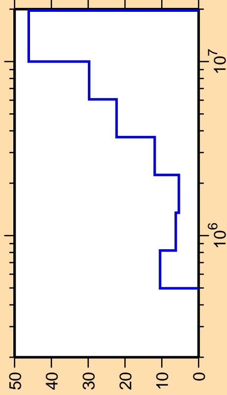
\Delta\sigma/\sigma vs. E for ^{65}\text{Zn}(n,n_4)
