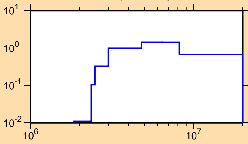
\sigma vs. E for ^{65}\text{Zn}(n,n\text{cont.})
