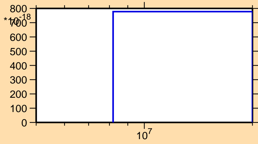
\sigma vs. E for ^{66}\text{Zn}(n,nt)
