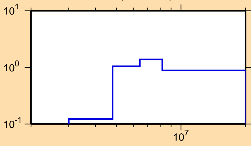
\sigma vs. E for ^{66}\text{Zn}(n,n\text{cont.})
