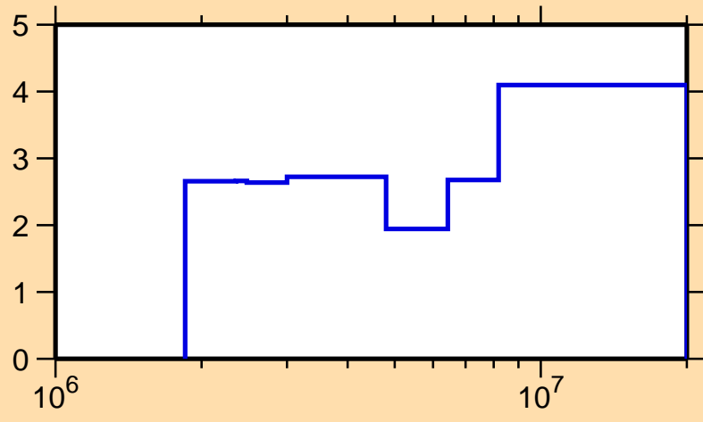
\Delta\sigma/\sigma vs. E for ^{66}\text{Zn}(n,el.)
