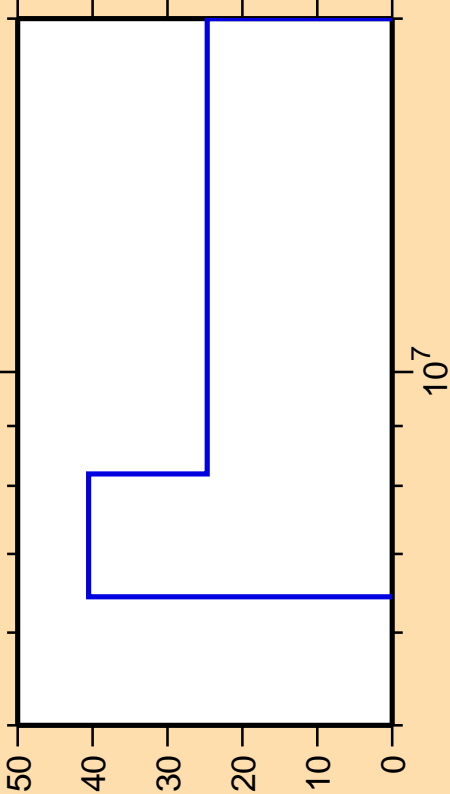
\Delta\sigma/\sigma vs. E for ^{66}\text{Zn}(n,n\alpha)
