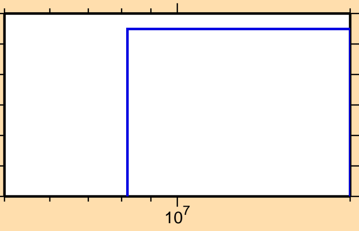
\sigma vs. E for ^{66}\text{Zn}(n,np)
