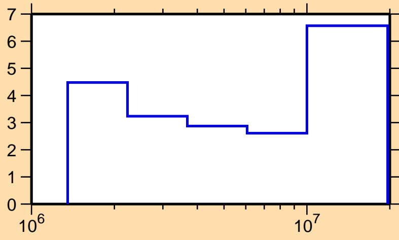
\Delta\sigma/\sigma vs. E for ^{67}\text{Zn}(n,n\text{cont.})
