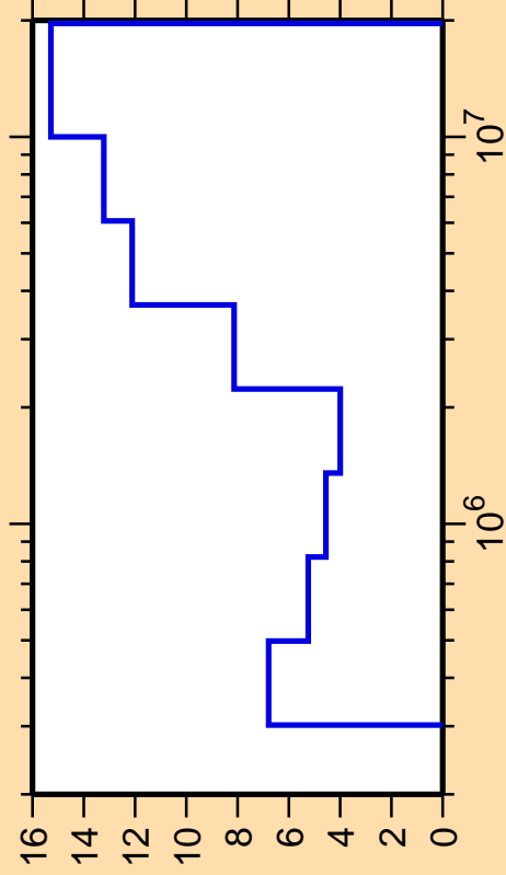
\Delta\sigma/\sigma vs. E for ^{67}\text{Zn}(n,n_3)
