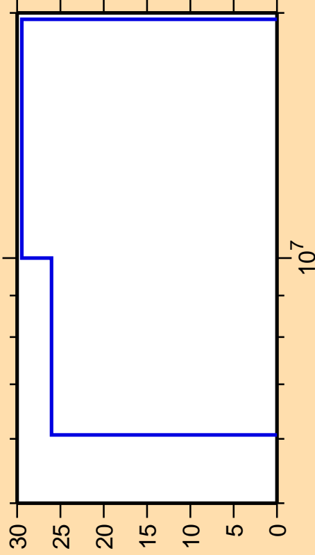
\Delta\sigma/\sigma vs. E for ^{67}\text{Zn}(n,\gamma)
