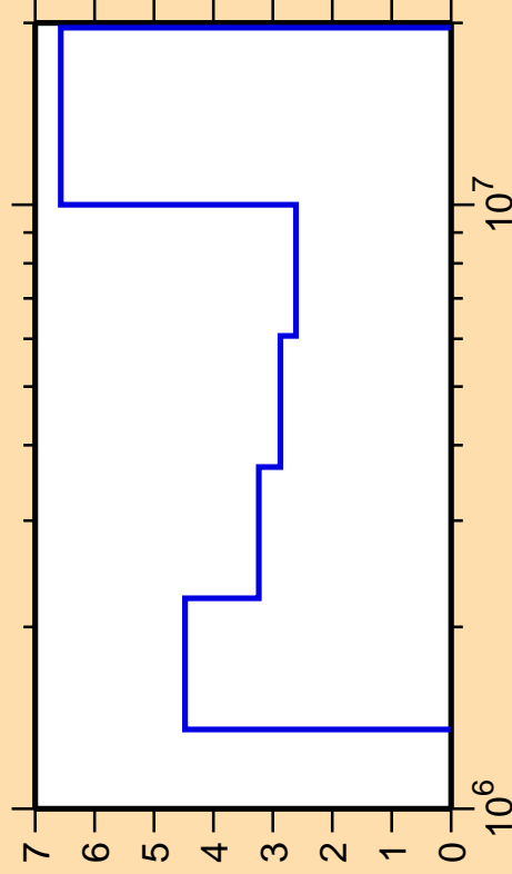
\Delta\sigma/\sigma vs. E for ^{67}\text{Zn}(n,n\text{cont.})
