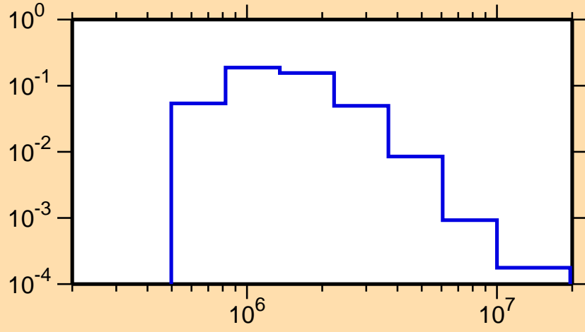
\sigma vs. E for ^{67}\text{Zn}(n,n_4)
