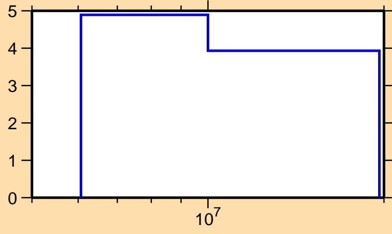
\Delta\sigma/\sigma vs. E for ^{67}\text{Zn}(n,2n)
