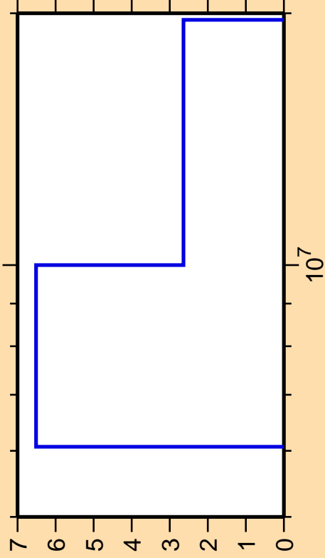
\Delta\sigma/\sigma vs. E for ^{67}\text{Zn}(n,\alpha)
