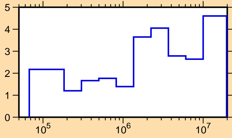
\Delta\sigma/\sigma vs. E for ^{67}\text{Zn}(n,\text{el.})
