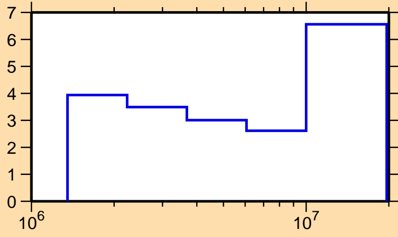
\Delta\sigma/\sigma vs. E for ^{67}\text{Zn}(n,\text{inel.})
