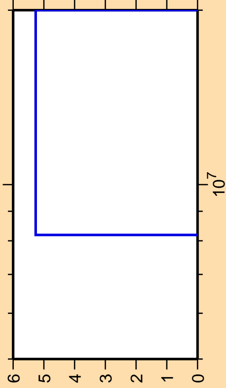
\Delta\sigma/\sigma vs. E for ^{67}\text{Zn}(n,\text{pt})
