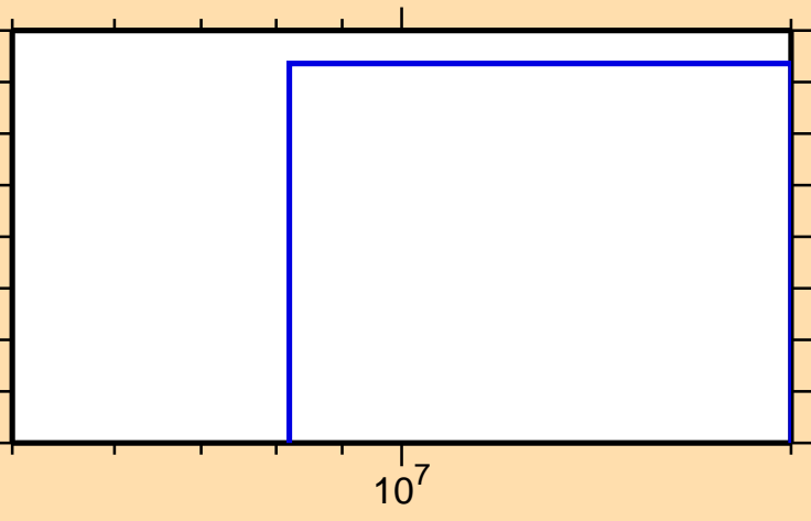
\sigma vs. E for ^{68}\text{Zn}(n,t)
