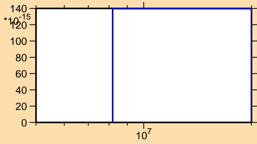
\sigma vs. E for ^{68}\text{Zn}(n,nt)
