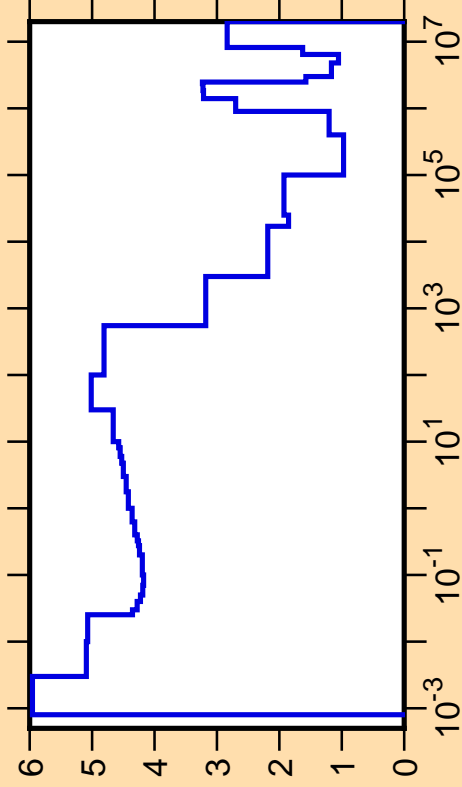
\Delta\sigma/\sigma vs. E for ^{68}\text{Zn}(n,\text{tot.})
