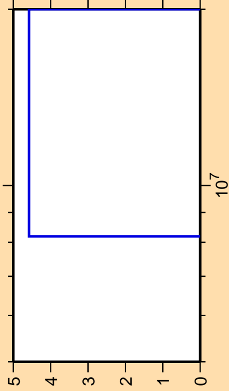
\Delta\sigma/\sigma vs. E for ^{68}\text{Zn}(n,2n)
