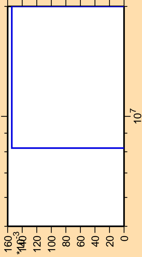
\Delta\sigma/\sigma vs. E for ^{68}\text{Zn}(n,nt)
