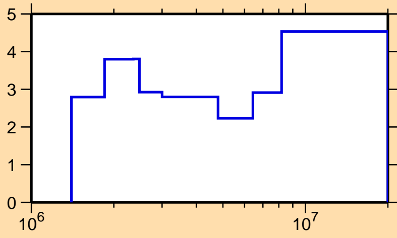
\Delta\sigma/\sigma vs. E for ^{68}\text{Zn}(n,\text{el.})
