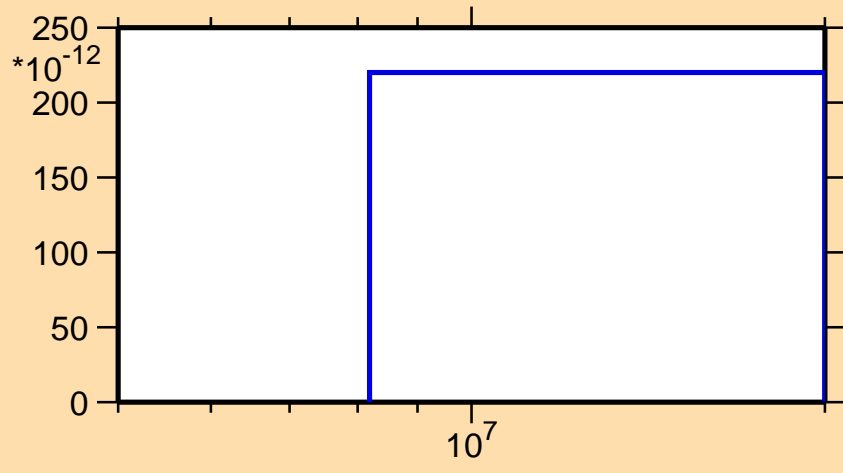
\sigma vs. E for ^{68}\text{Zn}(n,nd)
