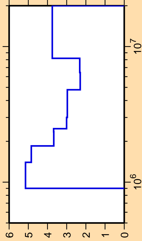
\Delta\sigma/\sigma vs. E for ^{68}\text{Zn}(n,\text{inel.})
