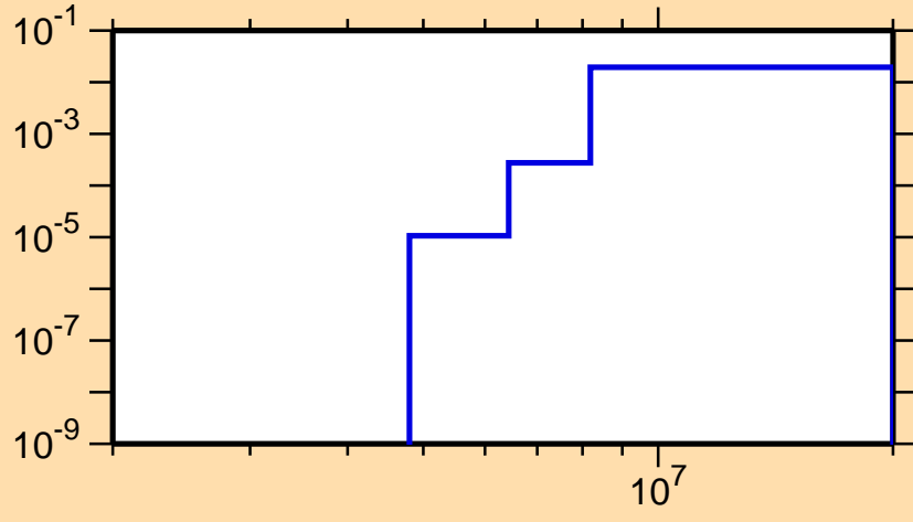
\sigma vs. E for ^{68}\text{Zn}(n,p)
