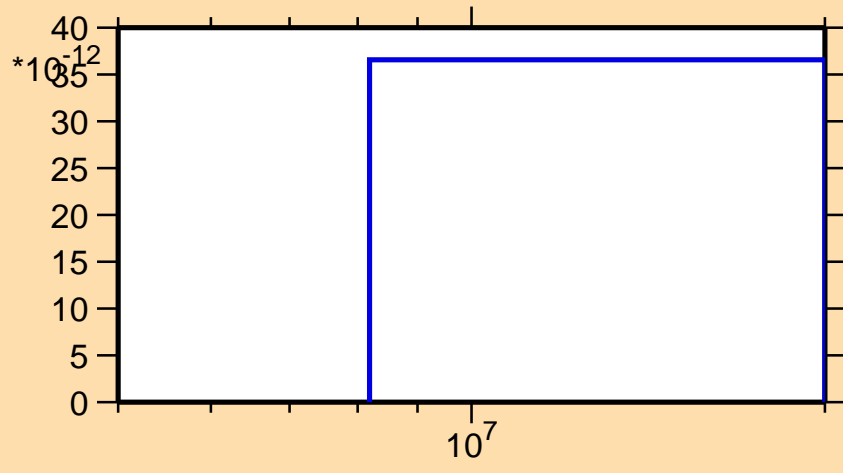
\sigma vs. E for ^{68}\text{Zn}(n,2n\alpha)
