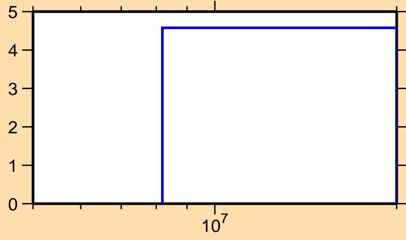
\Delta\sigma/\sigma vs. E for ^{68}\text{Zn}(n,2n)
