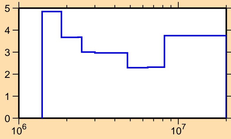
\Delta\sigma/\sigma vs. E for ^{68}\text{Zn}(n,\text{inel.})
