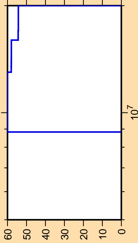
\Delta\sigma/\sigma vs. E for ^{70}\text{Zn}(n,d)
