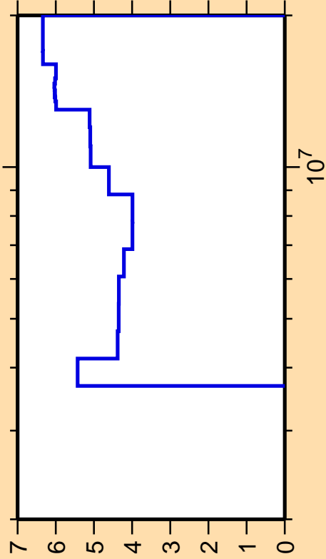
\Delta\sigma/\sigma vs. E for ^{70}\text{Zn}(n,n\text{cont.})
