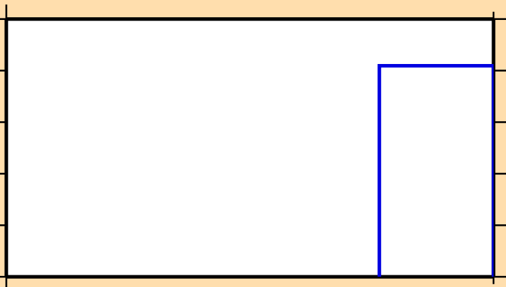
\sigma vs. E for ^{70}\text{Zn}(n,nd)
