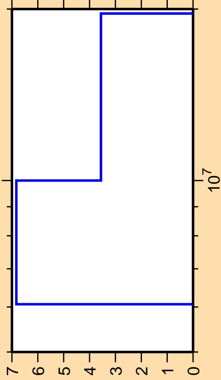
\Delta\sigma/\sigma vs. E for ^{70}\text{Zn}(n,2n)
