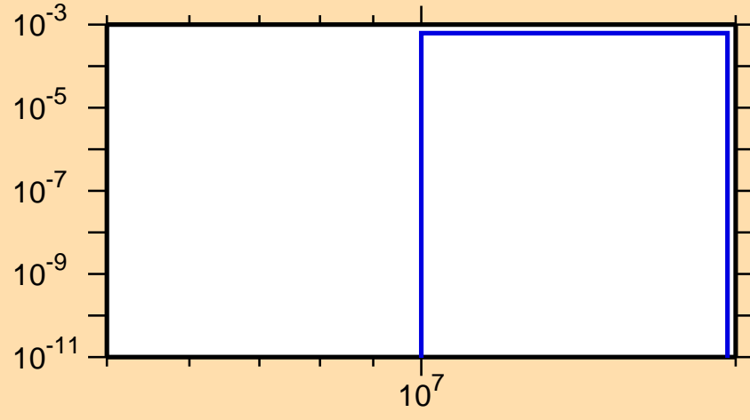
\sigma vs. E for ^{70}\text{Zn}(n,d)
