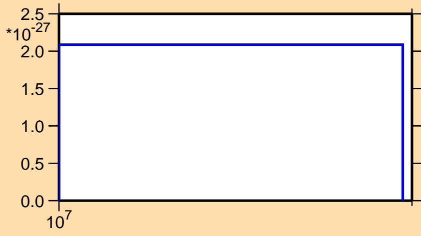
\sigma vs. E for ^{70}\text{Zn}(n,2np)
