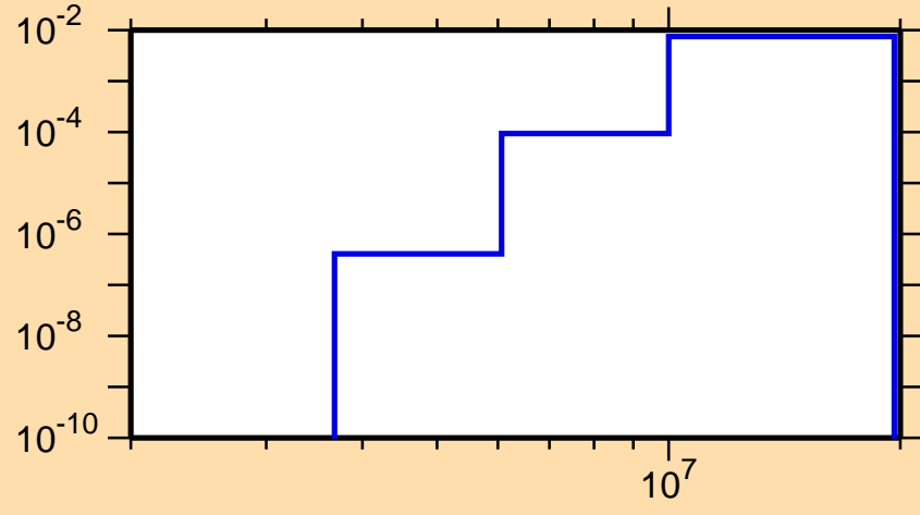
\sigma vs. E for ^{70}\text{Zn}(n,\alpha)
