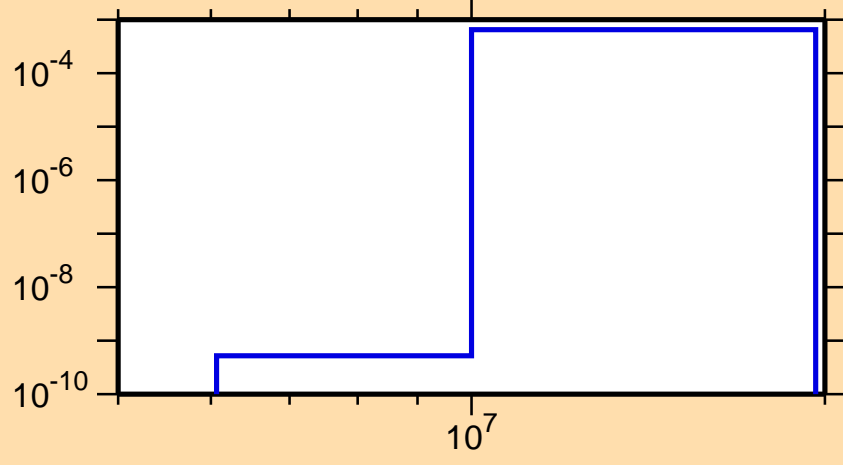
\sigma vs. E for ^{70}\text{Zn}(n,n\alpha)
