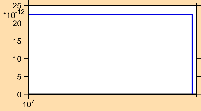
\sigma vs. E for ^{70}\text{Zn}(n,nd)
