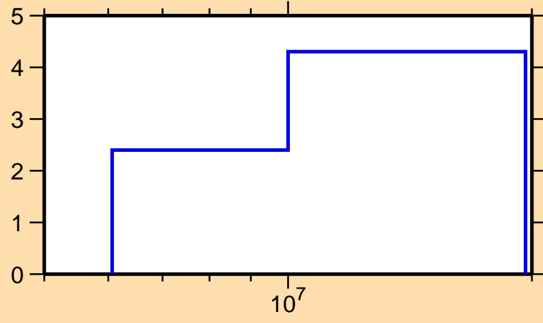
\Delta\sigma/\sigma vs. E for ^{70}\text{Zn}(n,\text{inel.})
