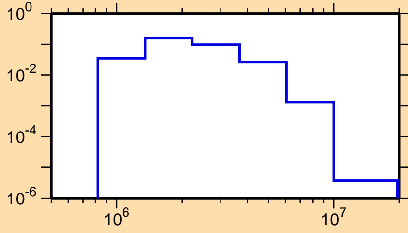
\sigma vs. E for ^{70}\text{Zn}(n,n_2)
