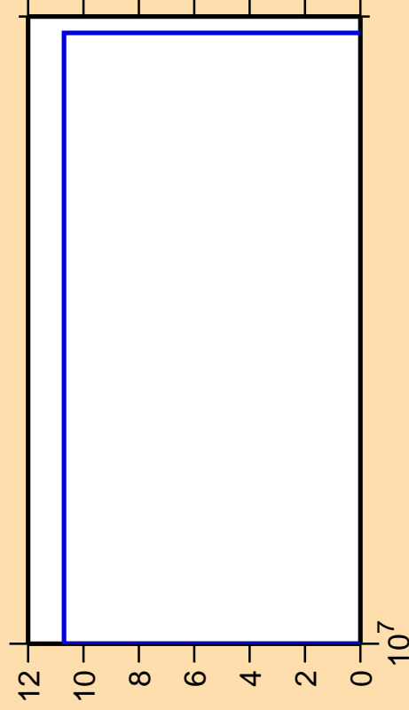
\Delta\sigma/\sigma vs. E for ^{70}\text{Zn}(n,nd)
