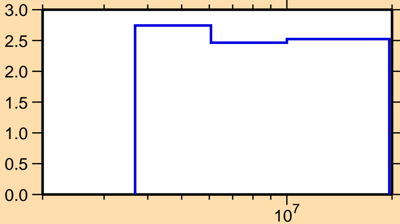
\Delta\sigma/\sigma vs. E for ^{70}\text{Zn}(n,n\text{onel.})
