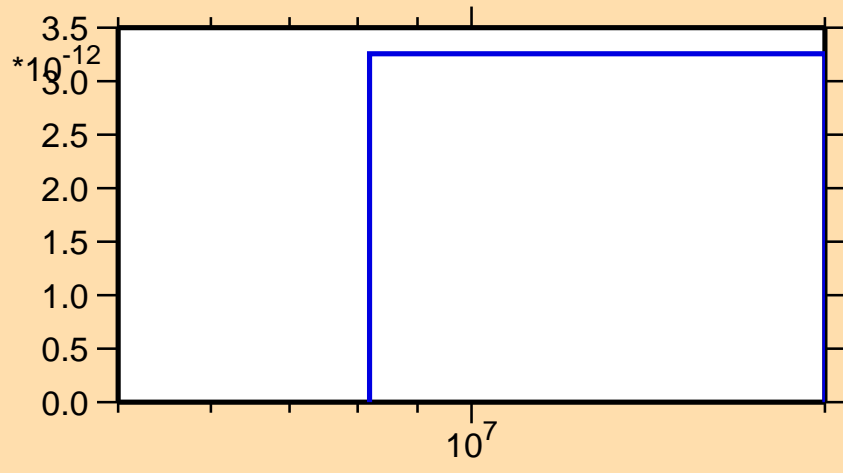
\sigma vs. E for ^{70}\text{Zn}(n,nt)
