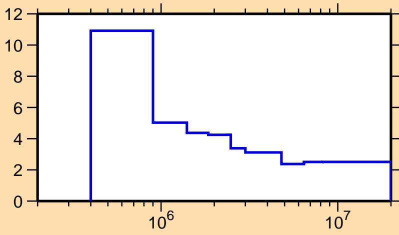
\Delta\sigma/\sigma vs. E for ^{70}\text{Zn}(n,\text{nonel.})
