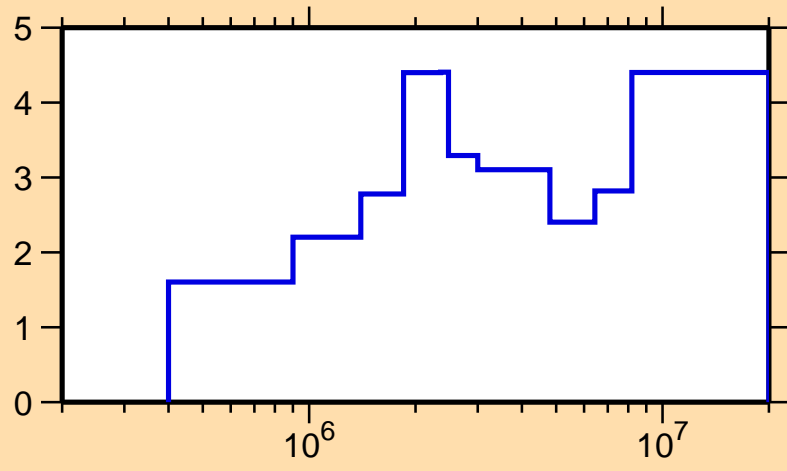
\Delta\sigma/\sigma vs. E for ^{70}\text{Zn}(n,\text{el.})
