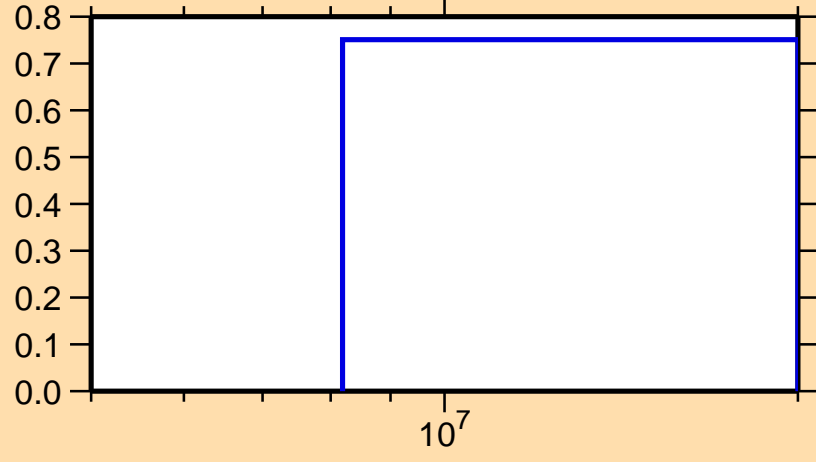
\sigma vs. E for ^{70}\text{Zn}(n,2n)
