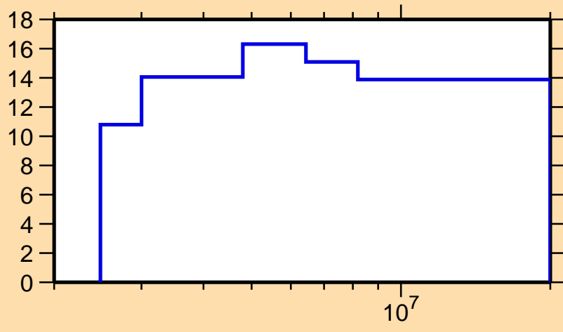
\Delta\sigma/\sigma vs. E for ^{70}\text{Zn}(n,n_1)
