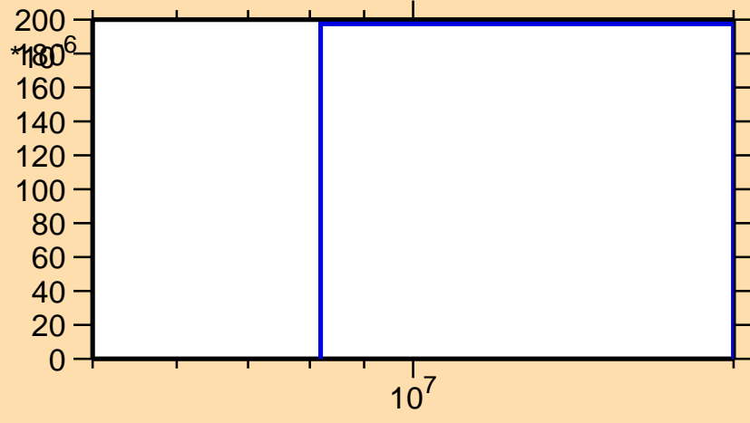
\sigma vs. E for ^{70}\text{Zn}(n,3n)
