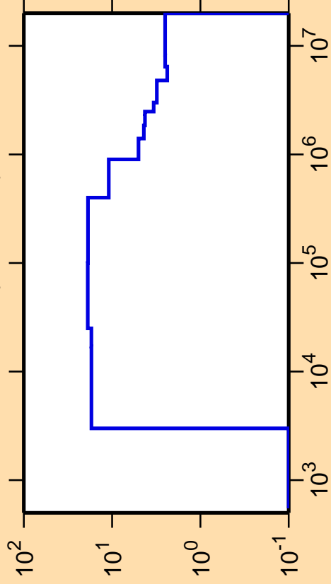
\Delta\sigma/\sigma vs. E for ^{70}\text{Zn}(n,\text{nonel.})
