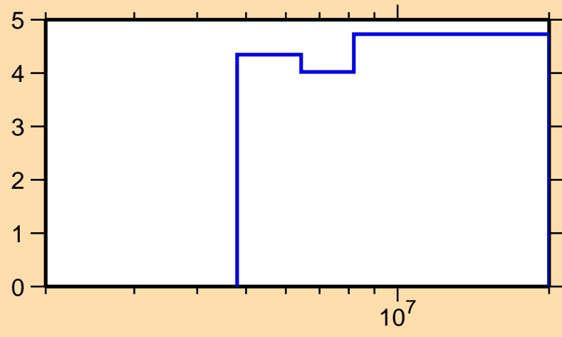
\Delta\sigma/\sigma vs. E for ^{70}\text{Zn}(n,n\text{cont.})
