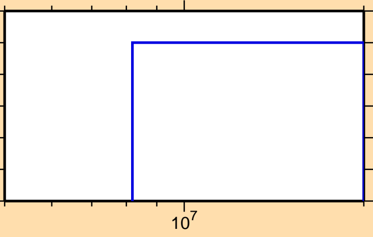
\sigma vs. E for ^{70}\text{Zn}(n,d)
