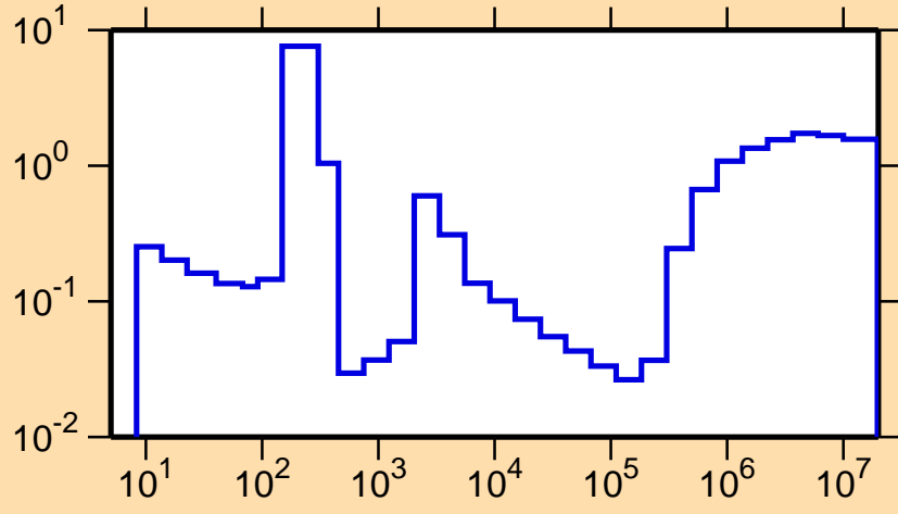
\sigma vs. E for ^{71}\text{Zn}(n,\text{nonel.})
