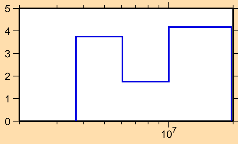
\Delta\sigma/\sigma vs. E for ^{71}\text{Zn}(n,\text{el.})
