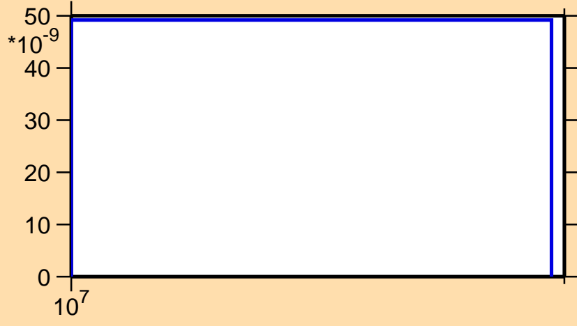
\sigma vs. E for ^{71}\text{Zn}(n,nd)
