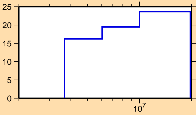
\Delta\sigma/\sigma vs. E for ^{71}\text{Zn}(n,p)
