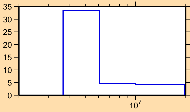
\Delta\sigma/\sigma vs. E for ^{71}\text{Zn}(n,2n)
