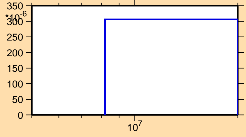
\sigma vs. E for ^{71}\text{Zn}(n,n\alpha)
