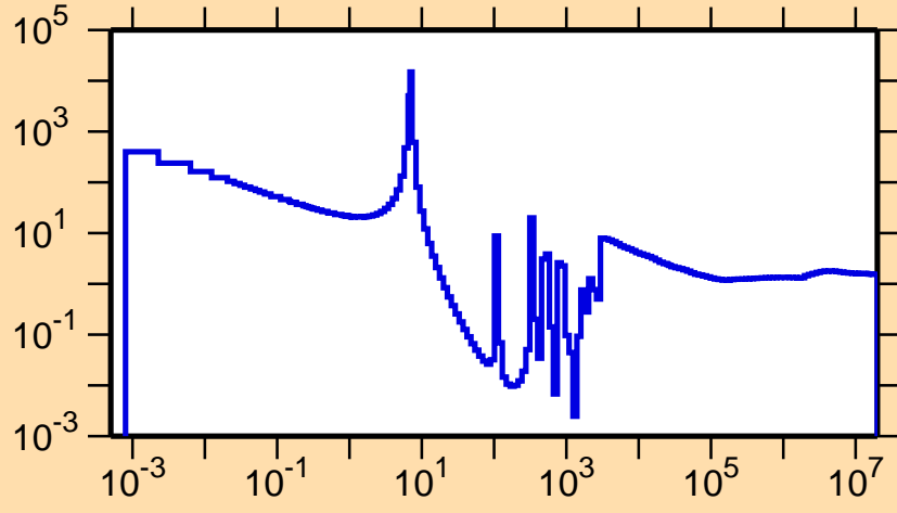
\sigma vs. E for ^{73}\text{Zn}(n,\text{nonel.})
