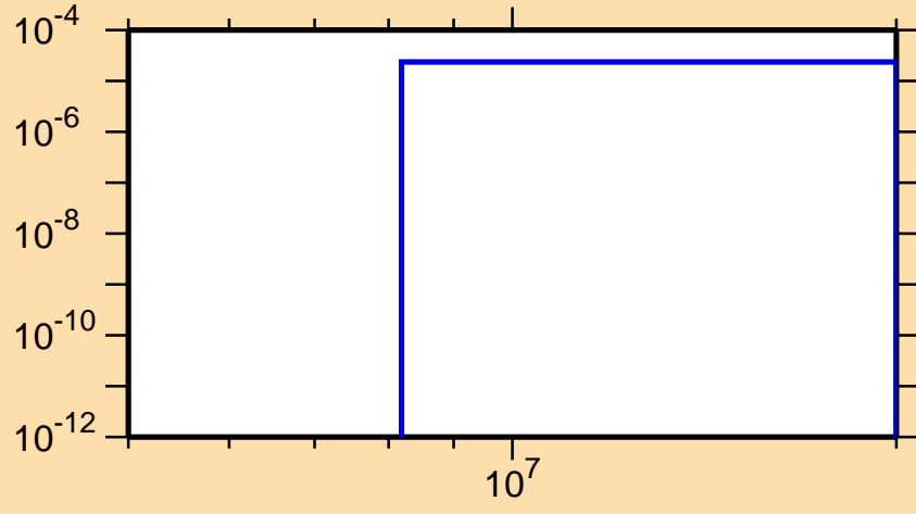
\sigma vs. E for ^{73}\text{Zn}(n,n\alpha)
