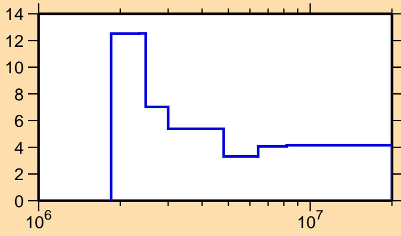
\Delta\sigma/\sigma vs. E for ^{73}\text{Zn}(n,n\text{onel.})
