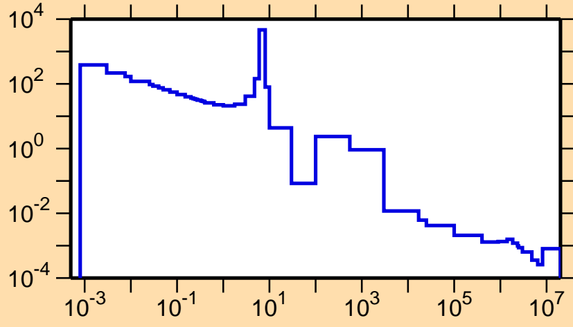
\sigma vs. E for ^{73}\text{Zn}(n,\gamma)
