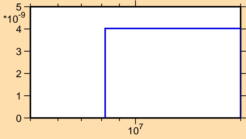
\sigma vs. E for ^{73}\text{Zn}(n,nd)
