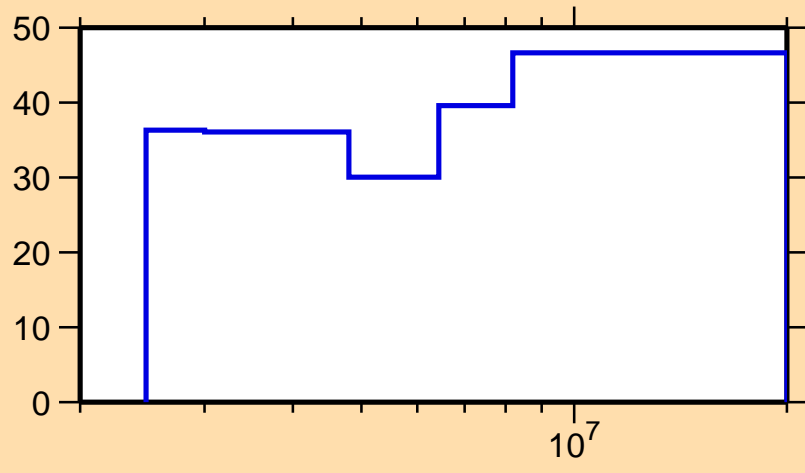
\Delta\sigma/\sigma vs. E for ^{73}\text{Zn}(n,\gamma)
