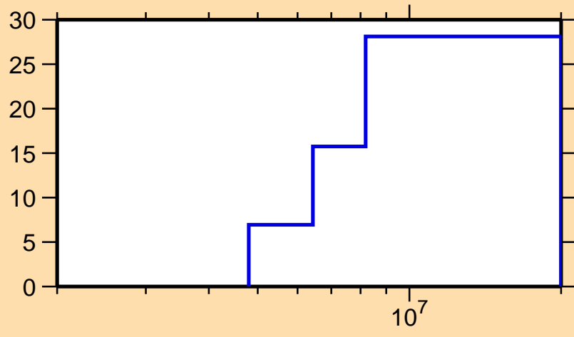
\Delta\sigma/\sigma vs. E for ^{73}\text{Zn}(n,n\text{cont.})
