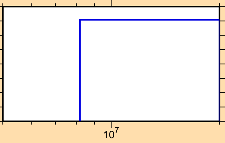
\sigma vs. E for ^{73}\text{Zn}(n,3n)
