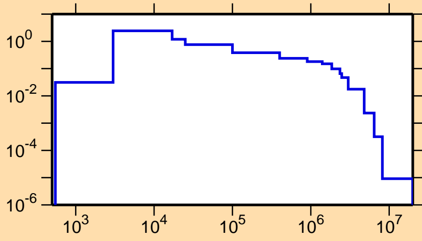
\sigma vs. E for ^{73}\text{Zn}(n,n_1)
