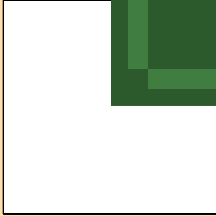
\sigma vs. E for ^{74}\text{Zn}(n,np)
