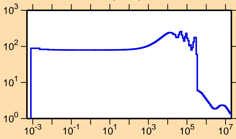
\sigma vs. E for ^{74}\text{Zn}(n,\text{el.})
