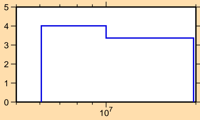
\Delta\sigma/\sigma vs. E for ^{74}\text{Zn}(n,\text{nonel.})
