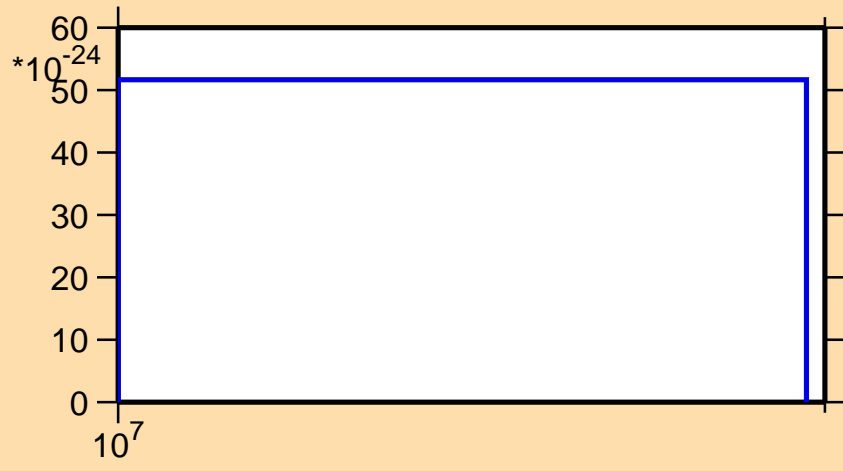
\sigma vs. E for ^{74}\text{Zn}(n,nd)
