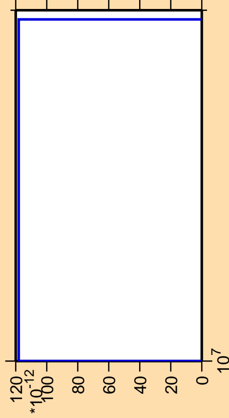
\Delta\sigma/\sigma vs. E for ^{74}\text{Zn}(n,nd)
