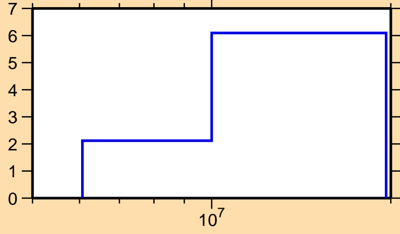
\Delta\sigma/\sigma vs. E for ^{74}\text{Zn}(n,\text{tot.})
