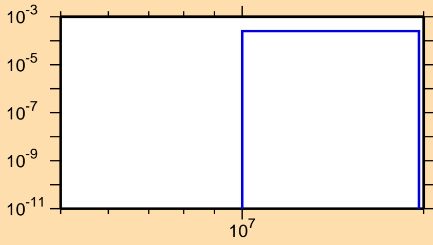
\sigma vs. E for ^{74}\text{Zn}(n,p)
