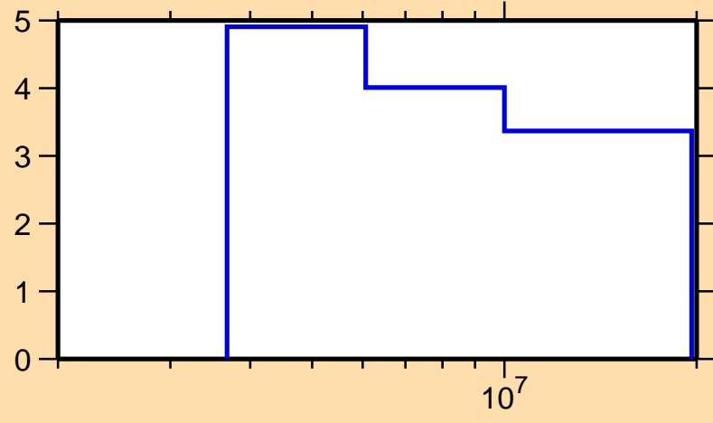
\Delta\sigma/\sigma vs. E for ^{74}\text{Zn}(n,n\text{onel.})
