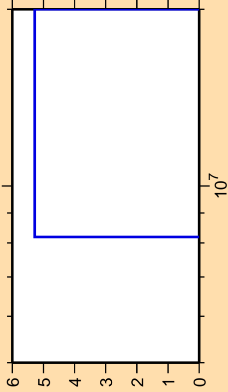
\Delta\sigma/\sigma vs. E for ^{74}\text{Zn}(n,2n)
