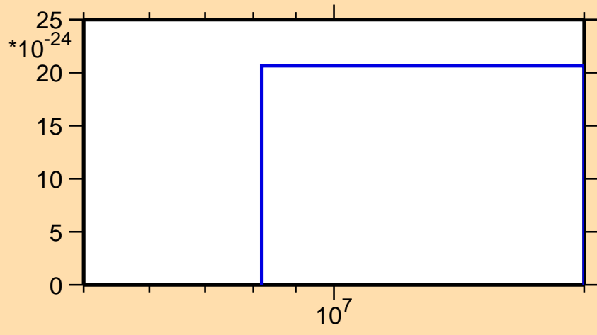
\sigma vs. E for ^{74}\text{Zn}(n,\text{He}3)
