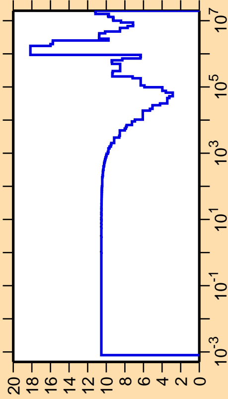
\Delta\sigma/\sigma vs. E for ^{78}\text{Zn}(n,\text{el.})
