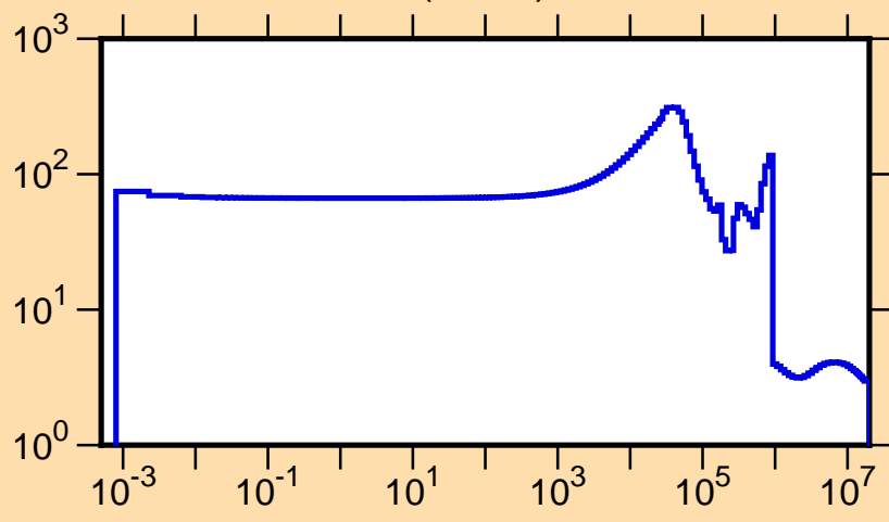
\sigma vs. E for ^{78}\text{Zn}(n,\text{tot.})
