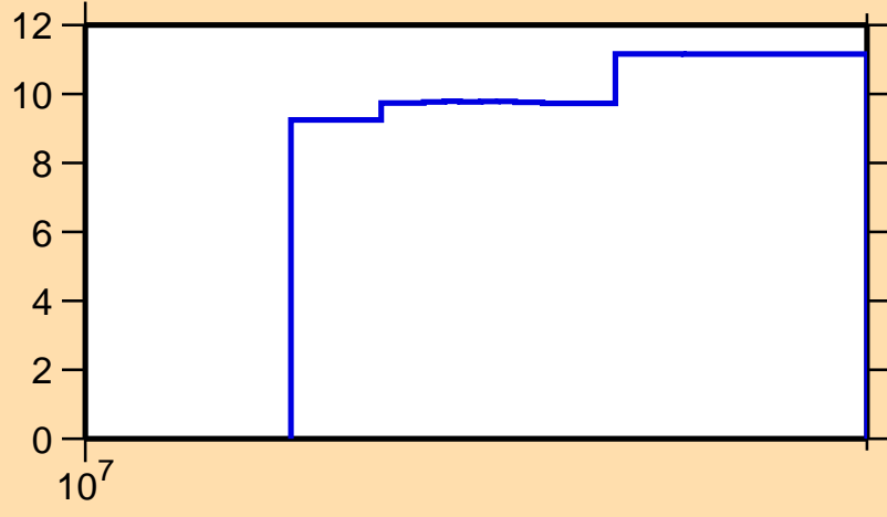
\Delta\sigma/\sigma vs. E for ^{78}\text{Zn}(n,el.)
