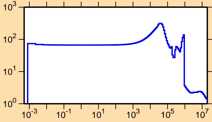
\sigma vs. E for ^{78}\text{Zn}(n,\text{el.})
