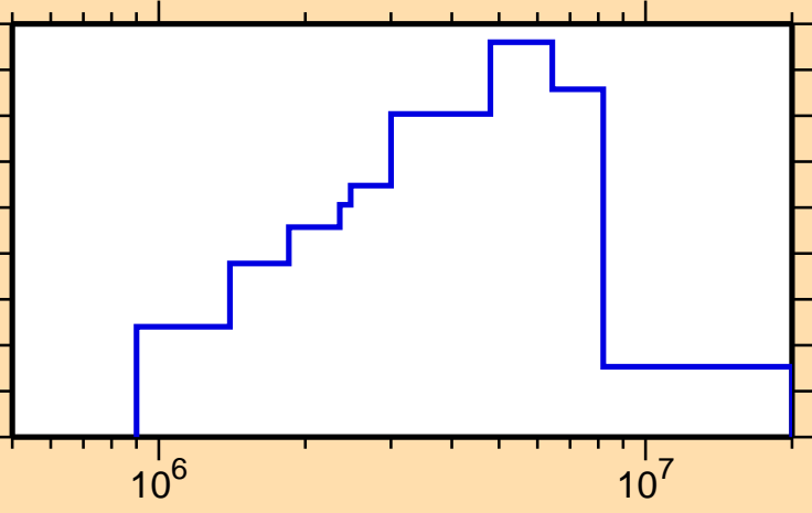
\sigma vs. E for ^{78}\text{Zn}(n,\text{inel.})
