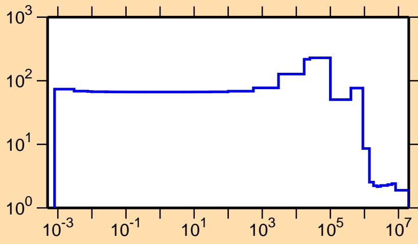
\sigma vs. E for ^{78}\text{Zn}(n,\text{el.})
