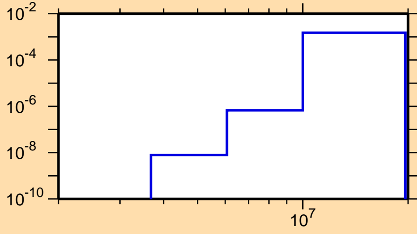
\sigma vs. E for ^{80}\text{Zr}(n,\text{He3})
