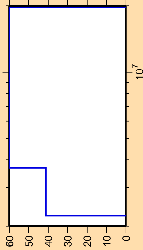
\Delta\sigma/\sigma vs. E for ^{80}\text{Zr}(n,n_4)
