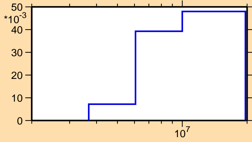
\sigma vs. E for ^{80}\text{Zr}(n,ncont.)
