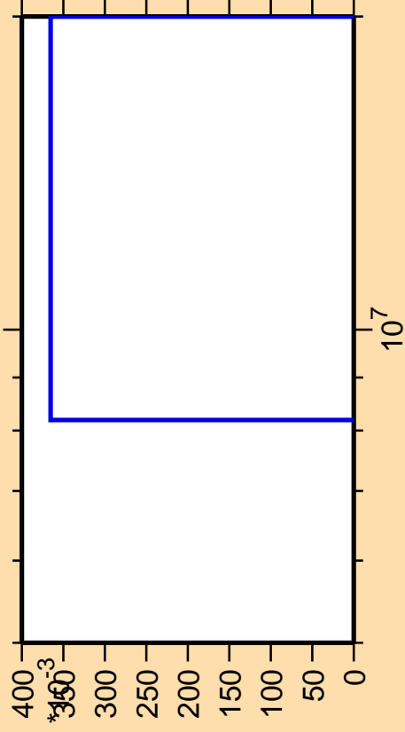
\Delta\sigma/\sigma vs. E for ^{80}\text{Zr}(n,\text{nd})
