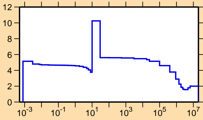
\sigma vs. E for ^{80}\text{Zr}(n,\text{el.})
