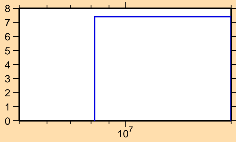
\Delta\sigma/\sigma vs. E for ^{80}\text{Zr}(n,\text{tot.})
