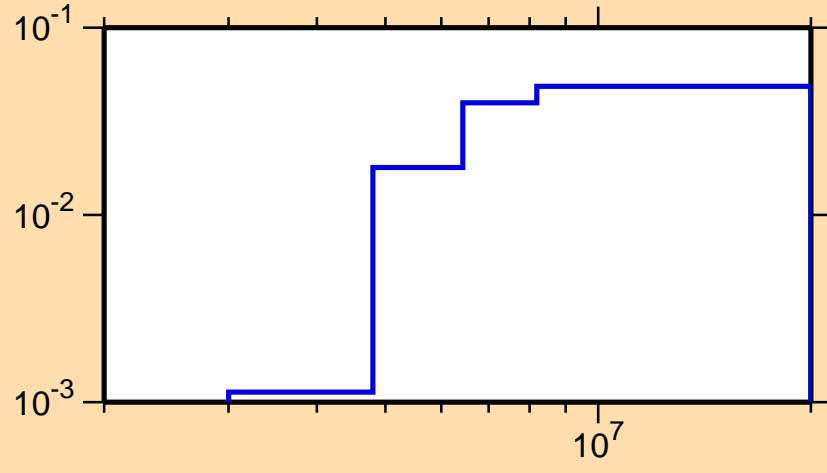
\sigma vs. E for ^{80}\text{Zr}(n,n\text{cont.})
