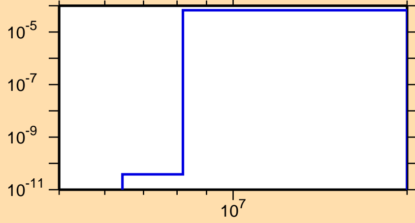
\sigma vs. E for ^{80}\text{Zr}(n,n\alpha)
