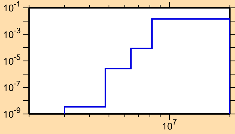
\sigma vs. E for ^{80}\text{Zr}(n,d)
