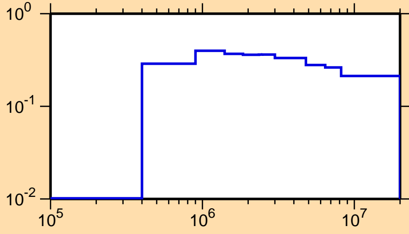
\sigma vs. E for ^{80}\text{Zr}(n,\text{inel.})
