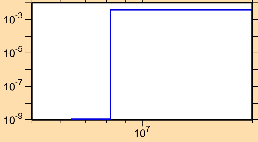
\sigma vs. E for ^{80}\text{Zr}(n,\text{pd})
